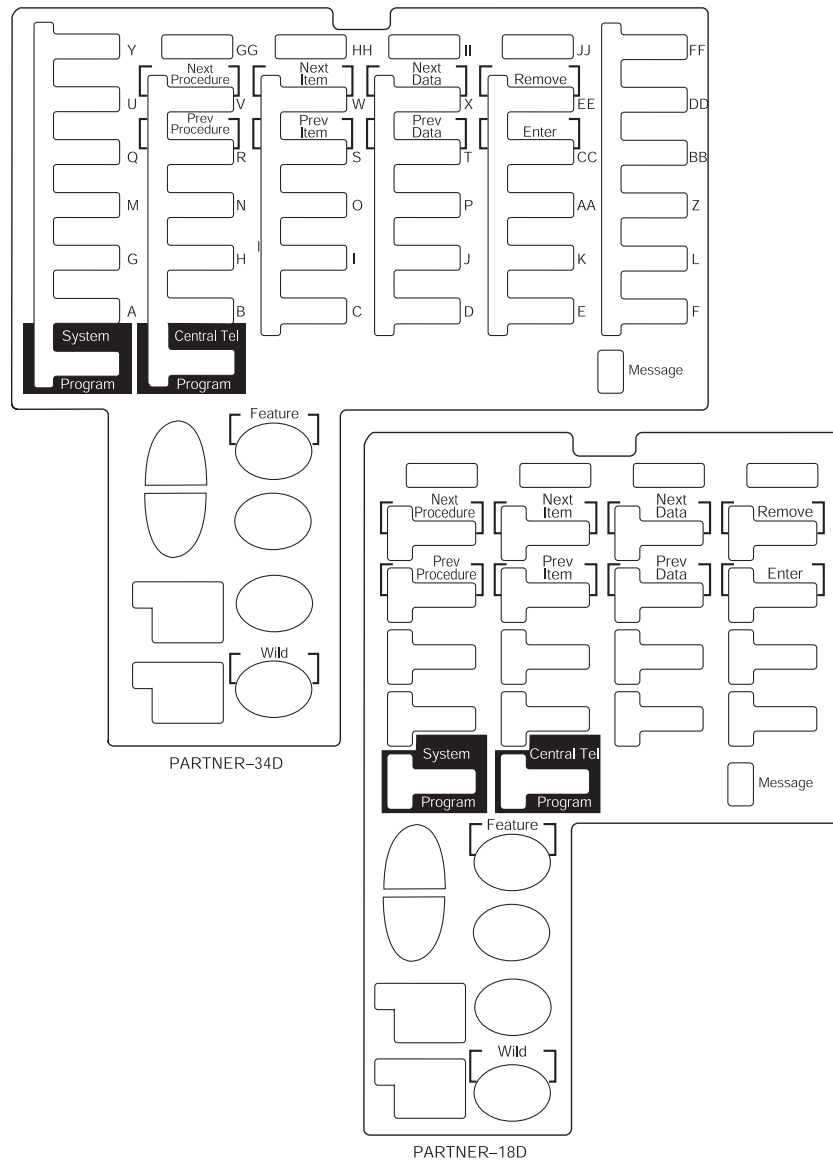
Figure 3-1. Programming Overlays
