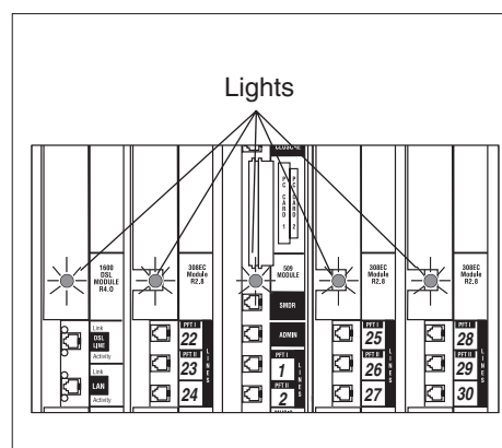
Figure 2-17. Module LEDs
