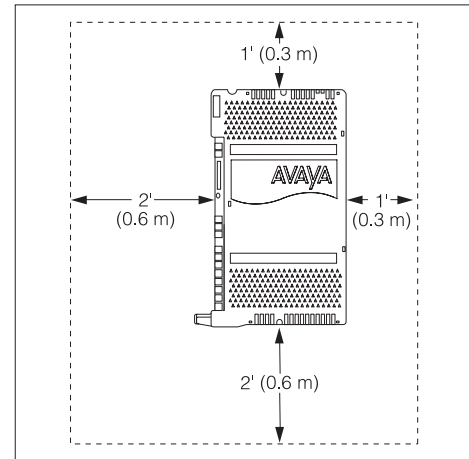
Figure 2-1. Processor Module Clearance
