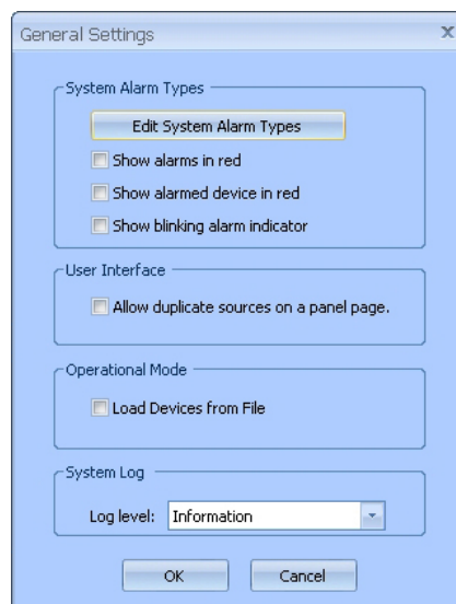
Figure 4-16 Cattrax General Settings Menu
