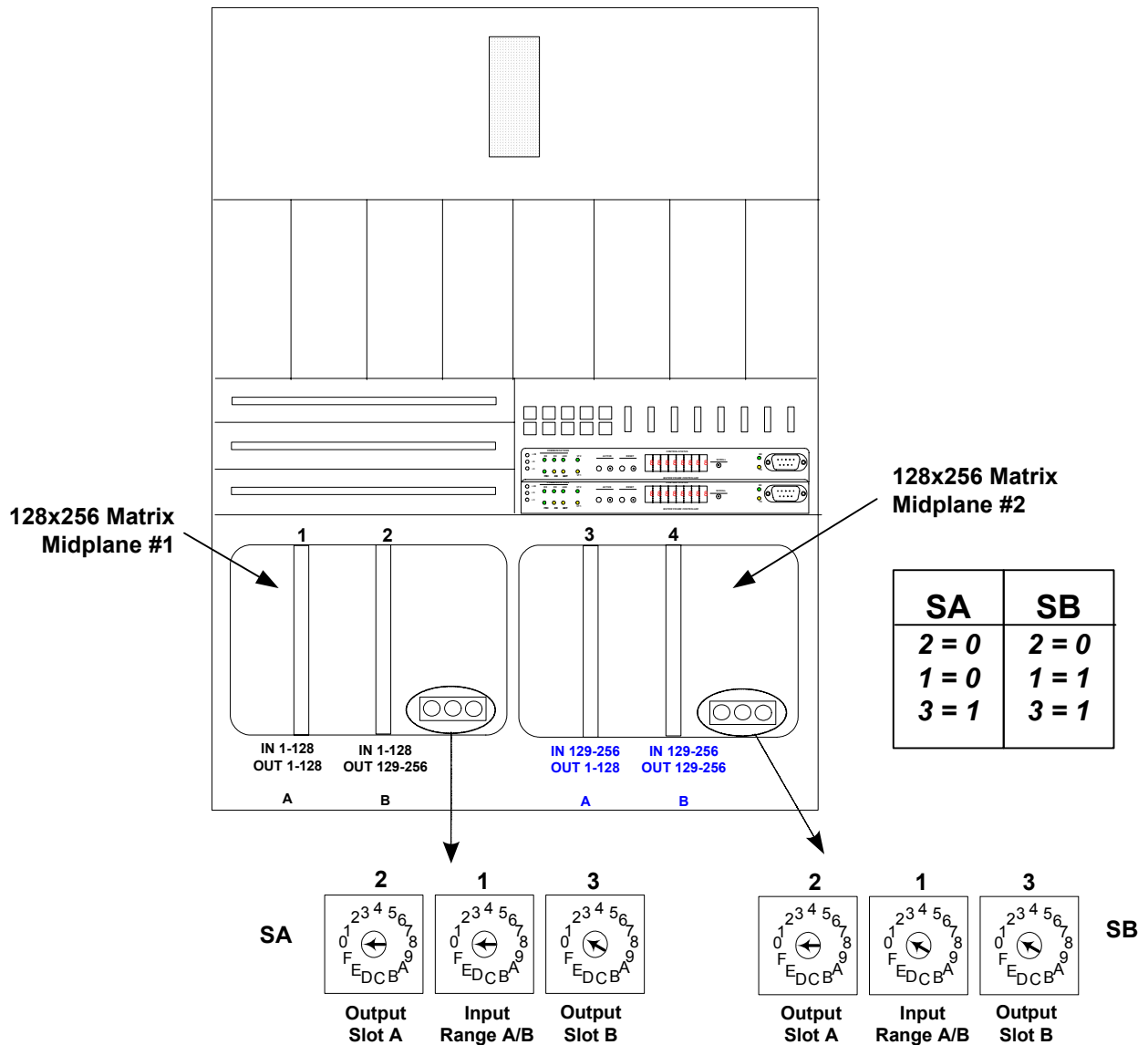
FIGURE 3-3: Matrix Backplane Rotary Switch Settings
