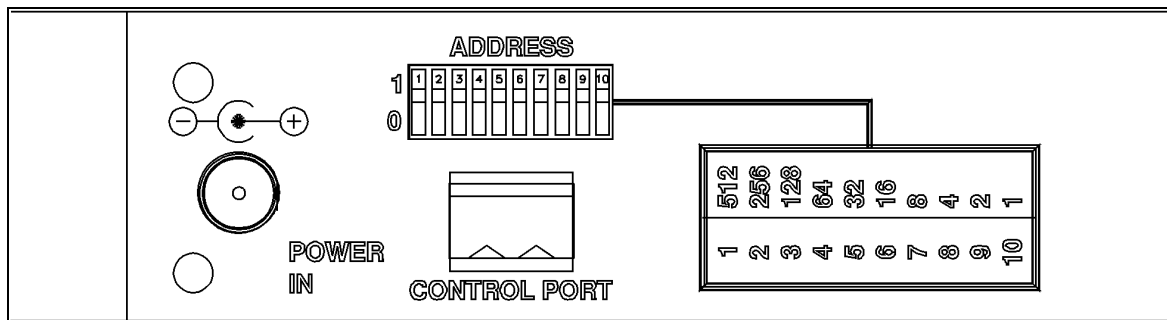
Figure 3-2. DIP Switch Location
