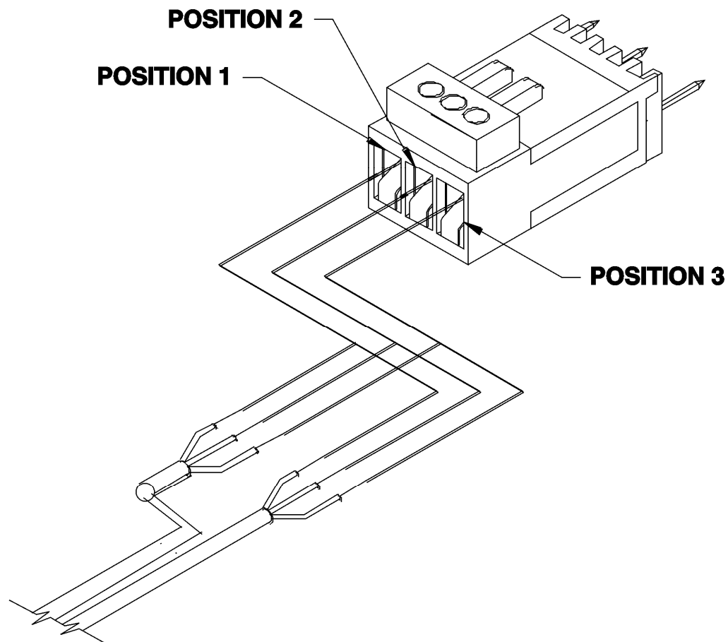
Figure 3-4. Wiring the Control Panel Connector
