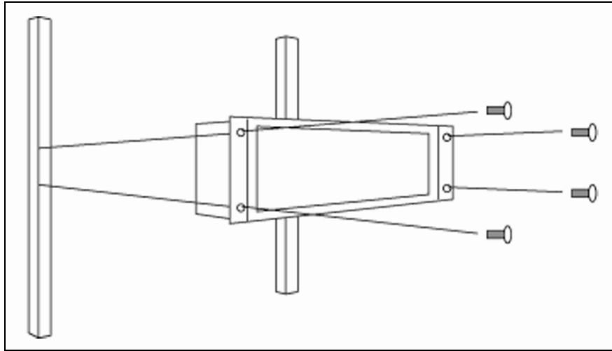
Figure 3-1. Remote Control Panel Installation
