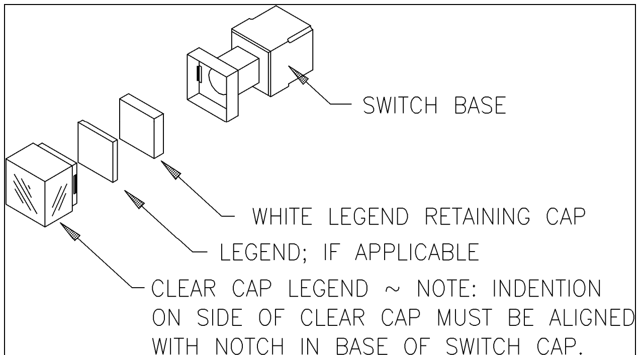
Figure 3-7. Switch Cap Assembly
