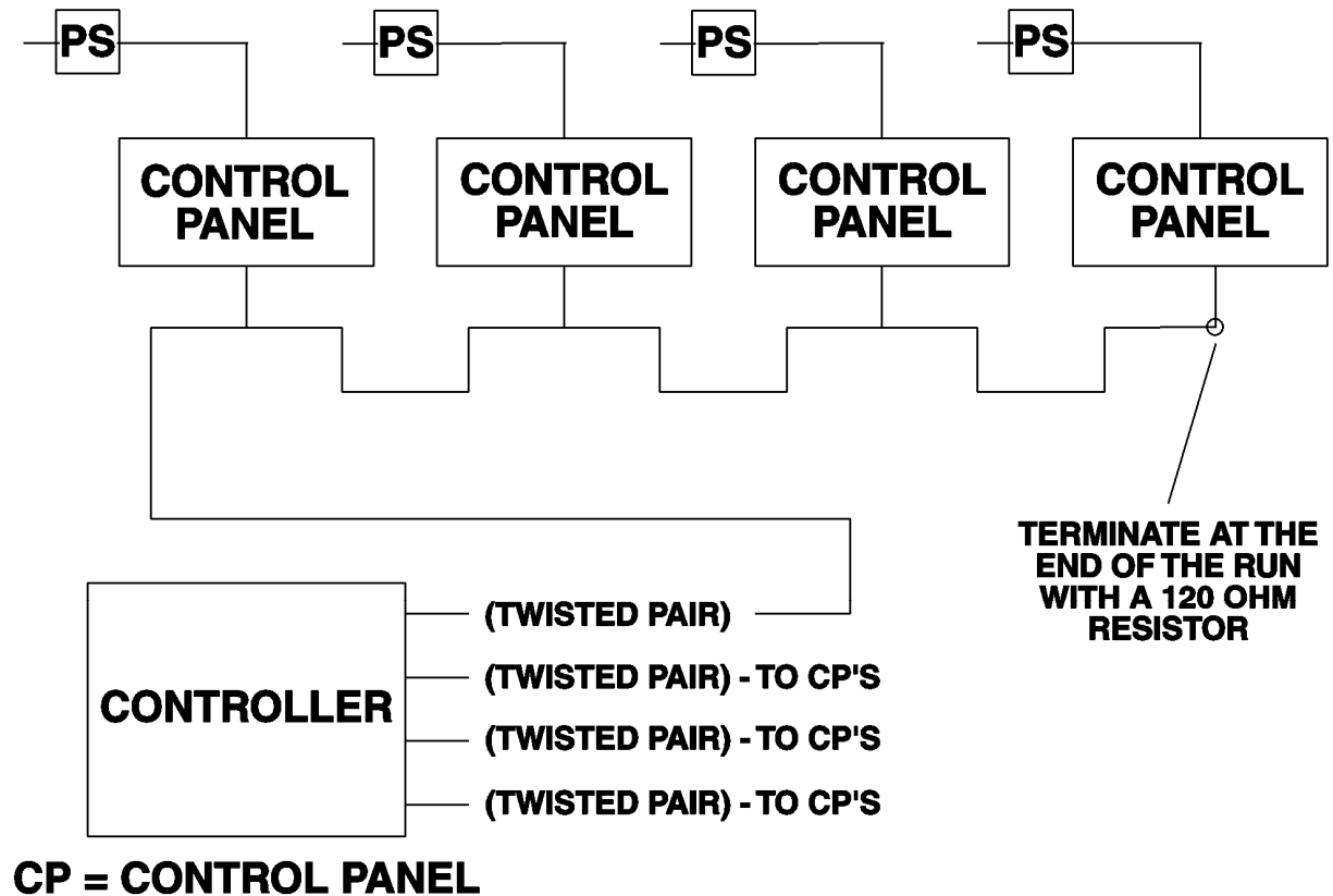
Figure 3-3. Typical Control Panel Interconnection
