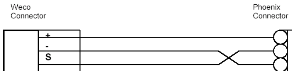
Figure 7. Pinout From Weco to Phoenix/Weidmuller
