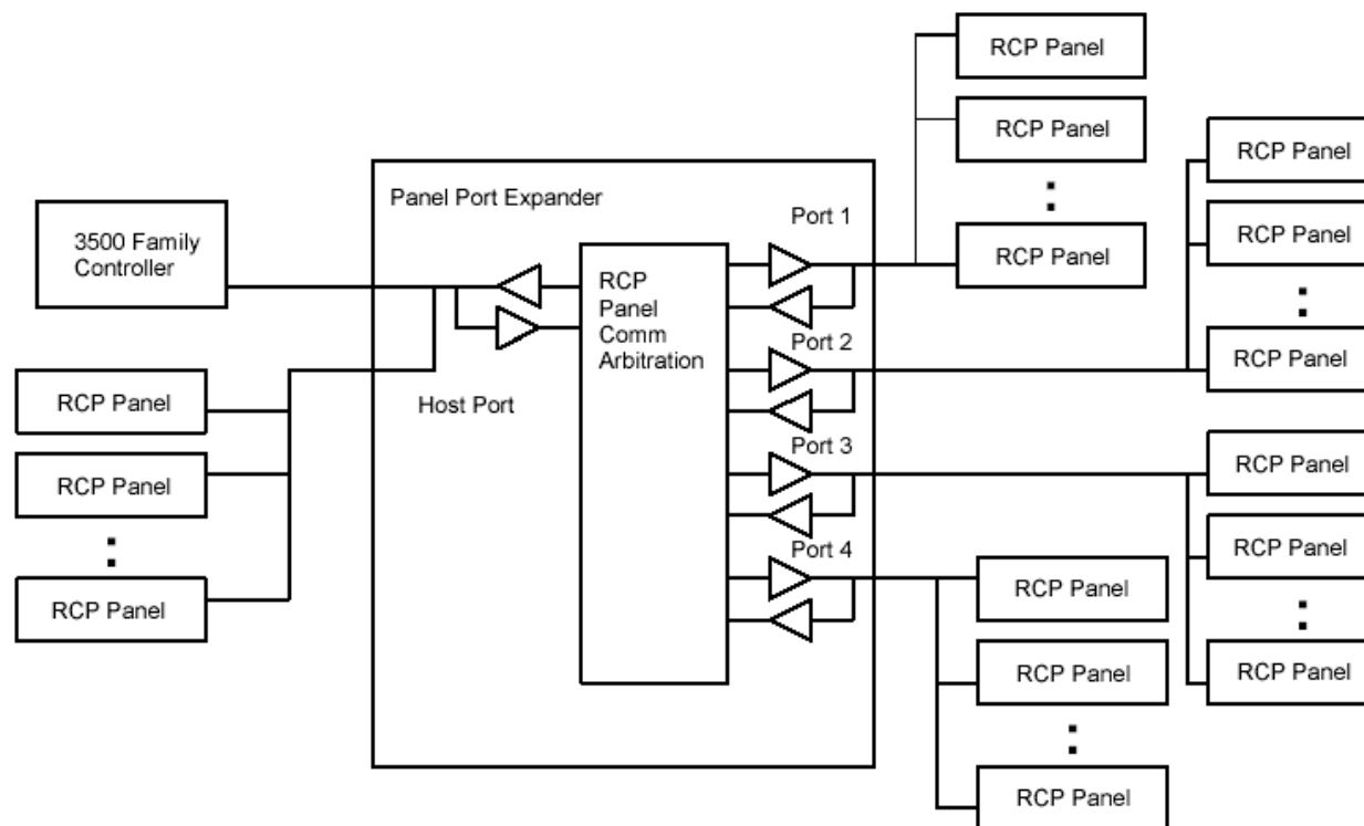
Figure 5. Dual 4x1 RCP Panel Port Expander Block Diagram
