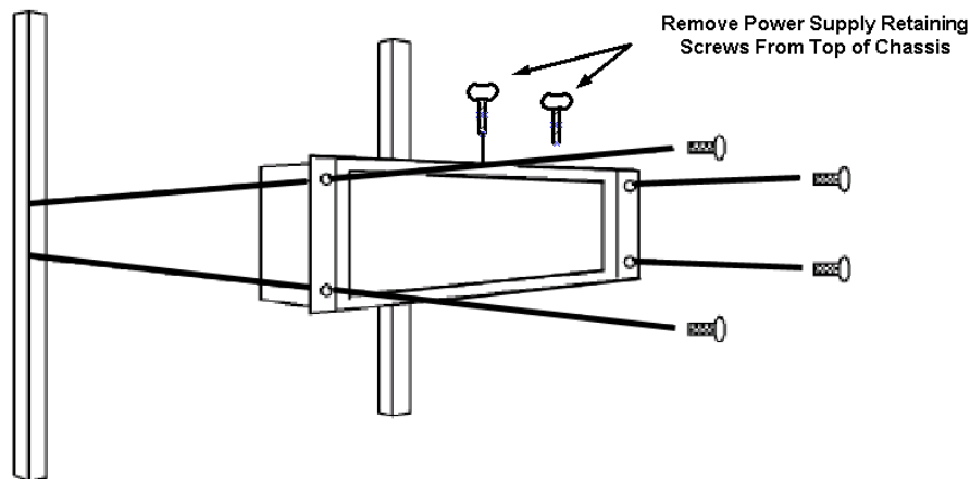
Figure 3. Chassis Installation
