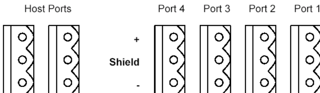
Figure 6. Rear Panel Connectors
