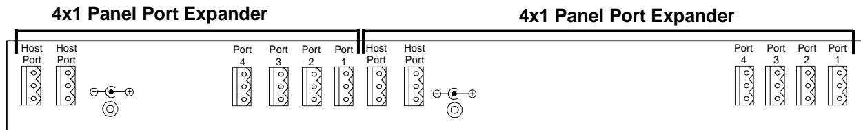
Figure 8. Dual 4x1 RCP Panel Port Expander Rear Panel Connectors
