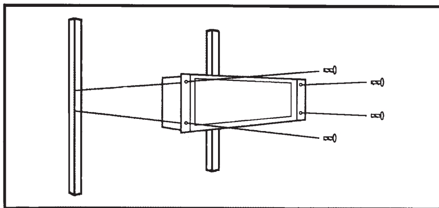
Figure 2-1 RCP-241 Chassis Installation
