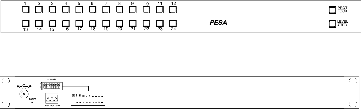
Figure 1-1 RCP-241 Front and Rear Views
