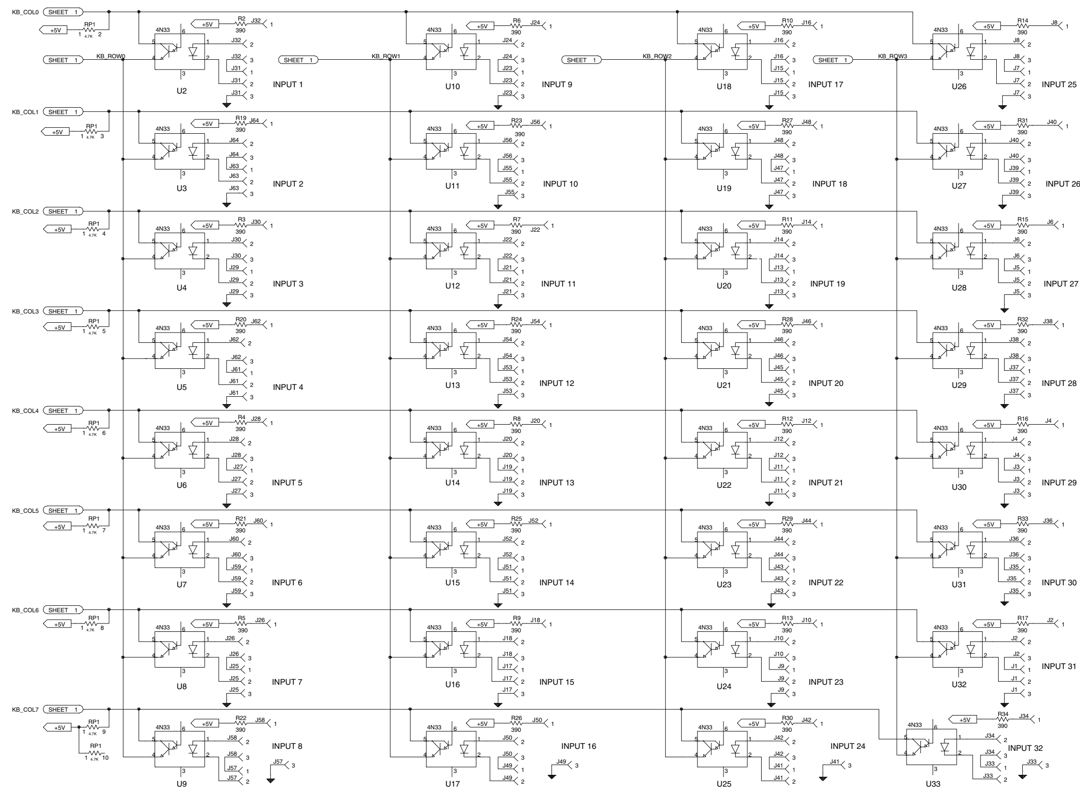
Schematic (Sheet 3 of 3) • RCP-GPIO Interface Card • SC33-1376
