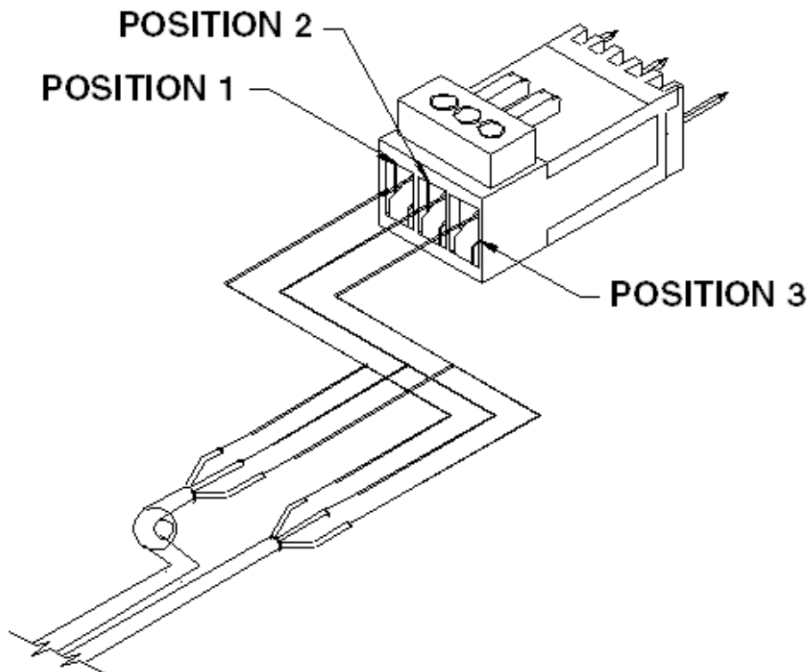
Figure 2-4 Wiring the Control Panel Connector
