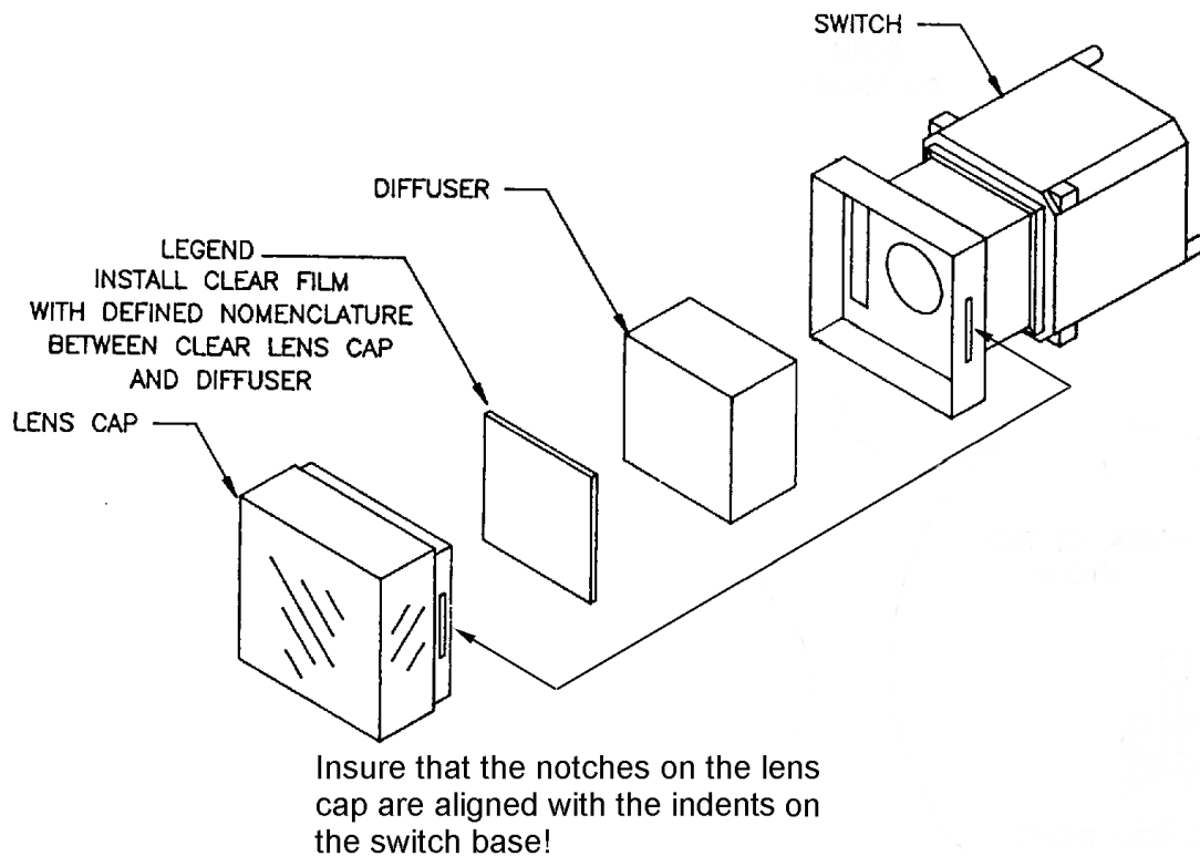
Figure 1-1 Pictorial View of Lens Cap Assembly
