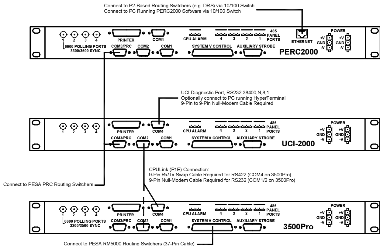
Figure 3 – Control Cable Connections
