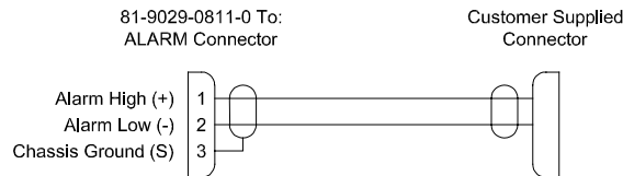
Figure 13. Alarm Switch Cable
