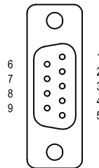
Contact locations when viewed from rear of chassis.
