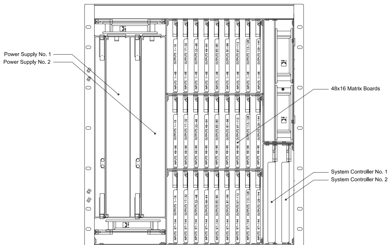
Figure 25. Front Subassemblies
