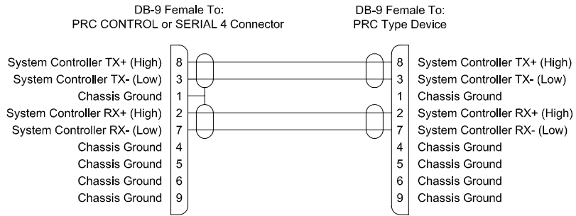
Figure 10. RS-422 Serial Cable
