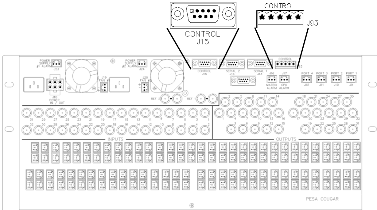
Figure 18. Control (PRC) Connectors (J15 and J93)
