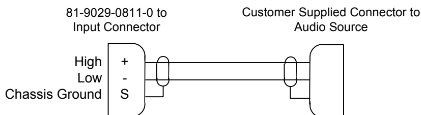
Figure 28. Input Signal Cable
