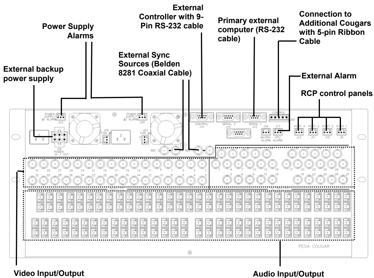
Figure 32. Connection Guide
