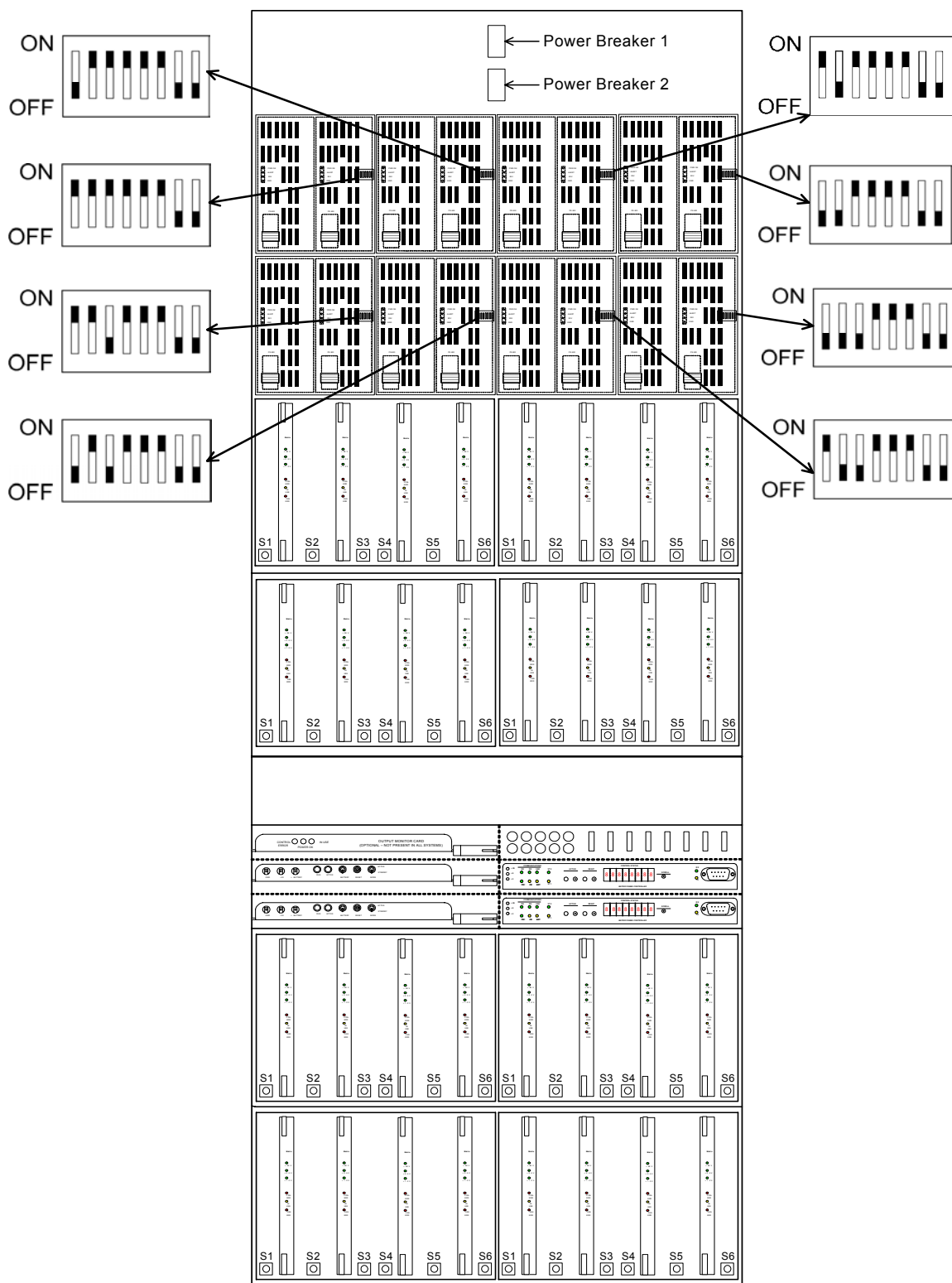
FIGURE 3-3: 1024X512 POWER SUPPLY BACKPLANE DIP SWITCH LOCATIONS AND SETTINGS (FRONT VIEW)
