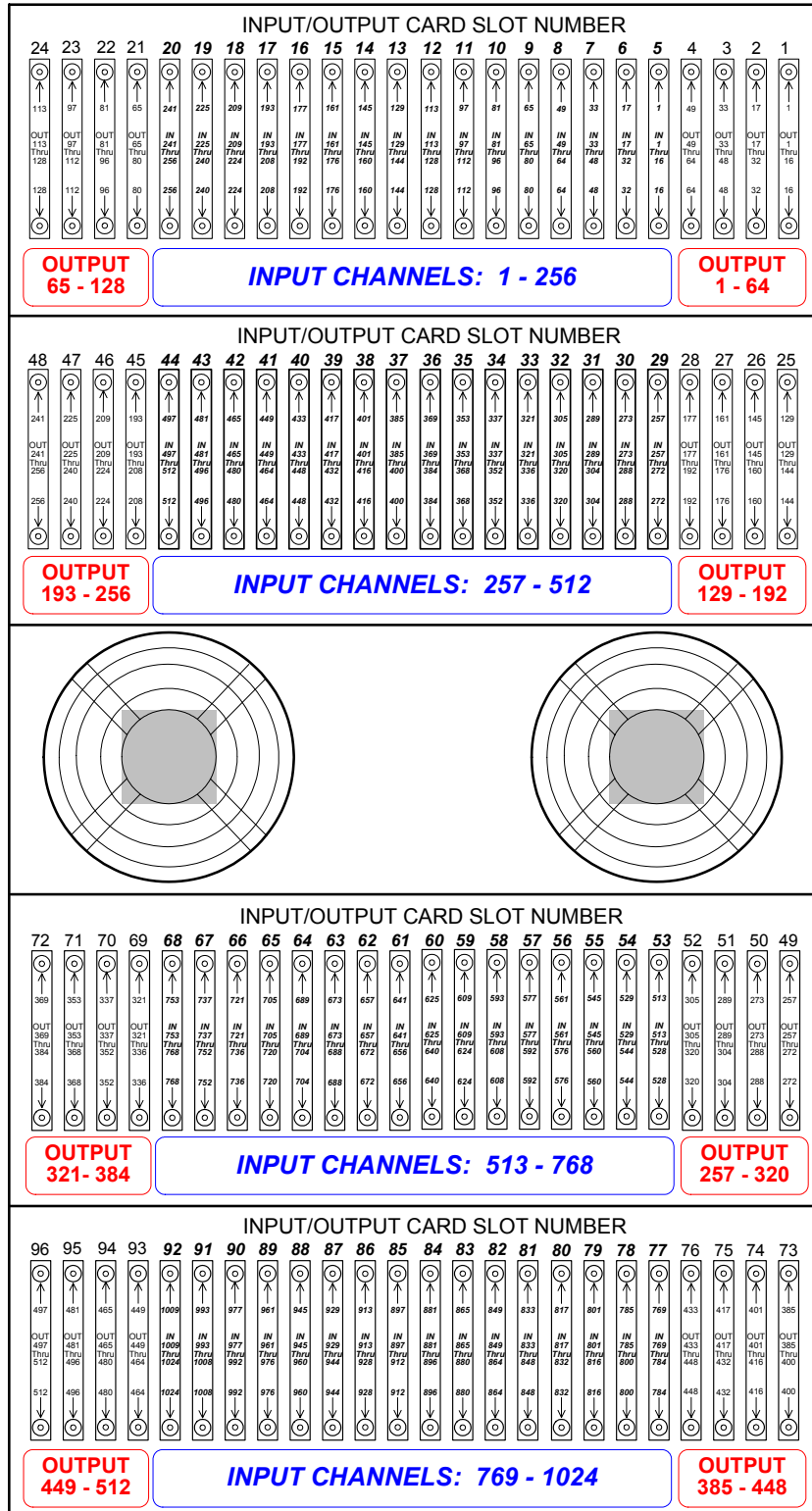
FIGURE 2-1: 1024X512 Router Input/Output Connector Arrangement
