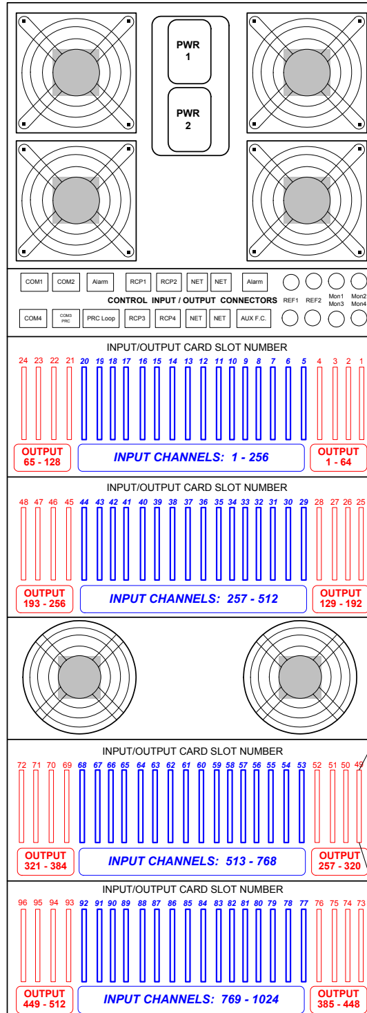
FIGURE 1-5: 1024X512 ROUTER CHASSIS (REAR VIEW)
