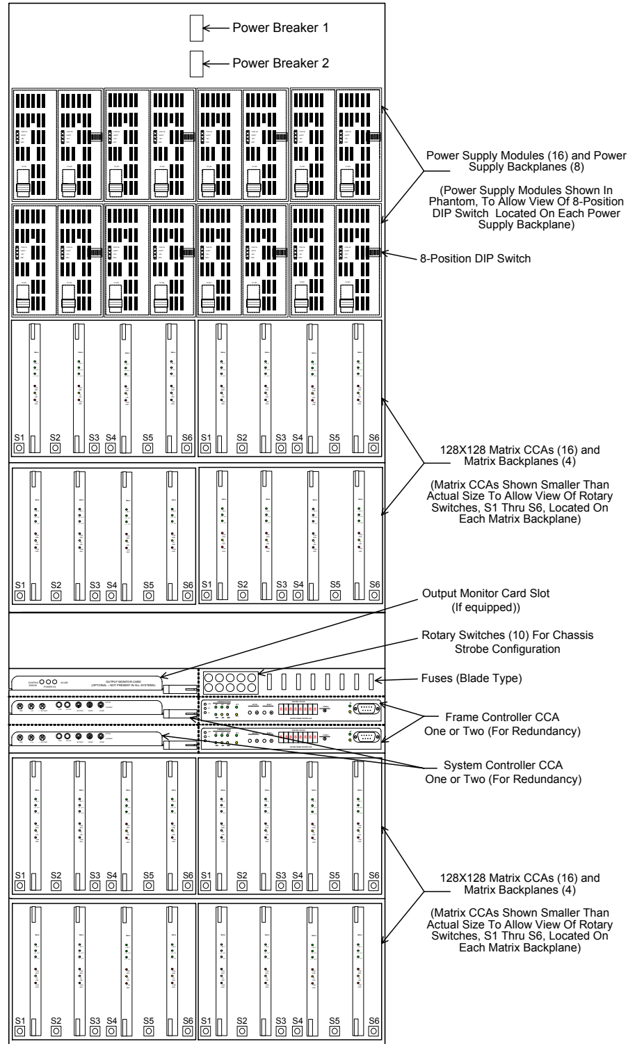
FIGURE 1-4 1024X512 ROUTER CHASSIS (FRONT VIEW – DOOR OPEN)
