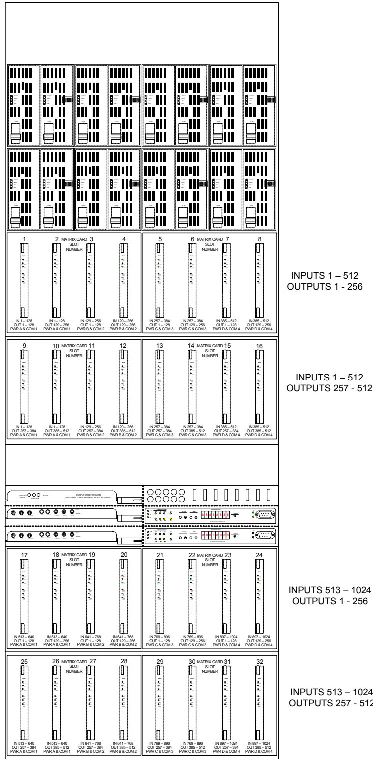
FIGURE 3-1: 128x128 MATRIX CROSSPOINT CCA I/O CHANNEL ASSIGNMENTS
