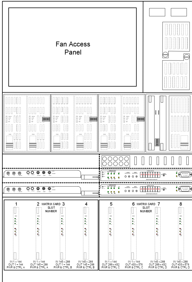
FIGURE 3-1: 288x576XE MATRIX CROSSPOINT CCA I/O CHANNEL ASSIGNMENTS
