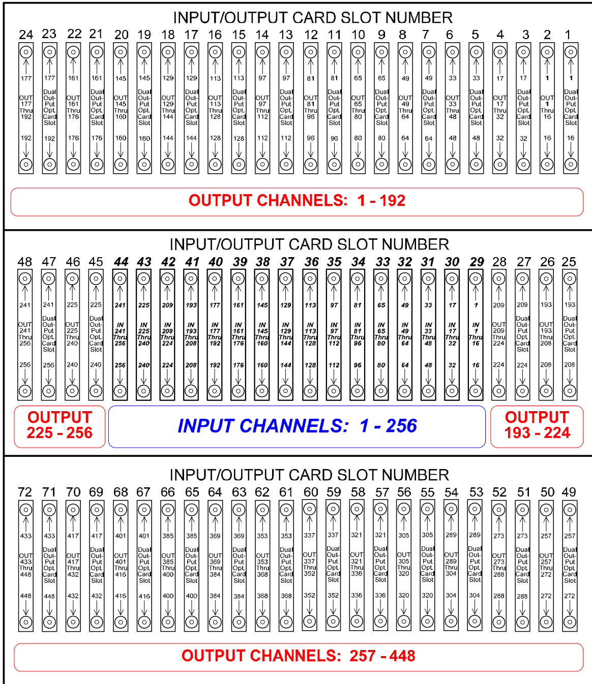
FIGURE 2-1: 256X448CX ROUTER INPUT/OUTPUT CONNECTOR ARRANGEMENT
