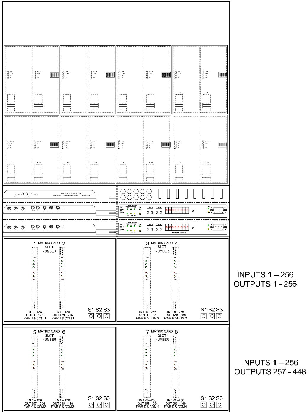
FIGURE 3-1: 256X448CX MATRIX CROSSPOINT CCA I/O CHANNEL ASSIGNMENTS
