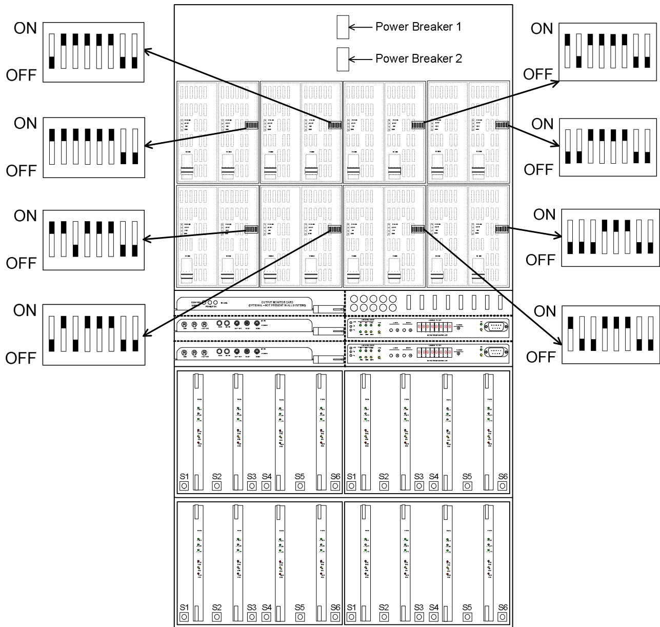
FIGURE 3-3: 576XR POWER SUPPLY BACKPLANE DIP SWITCH LOCATIONS AND SETTINGS (FRONT VIEW)
