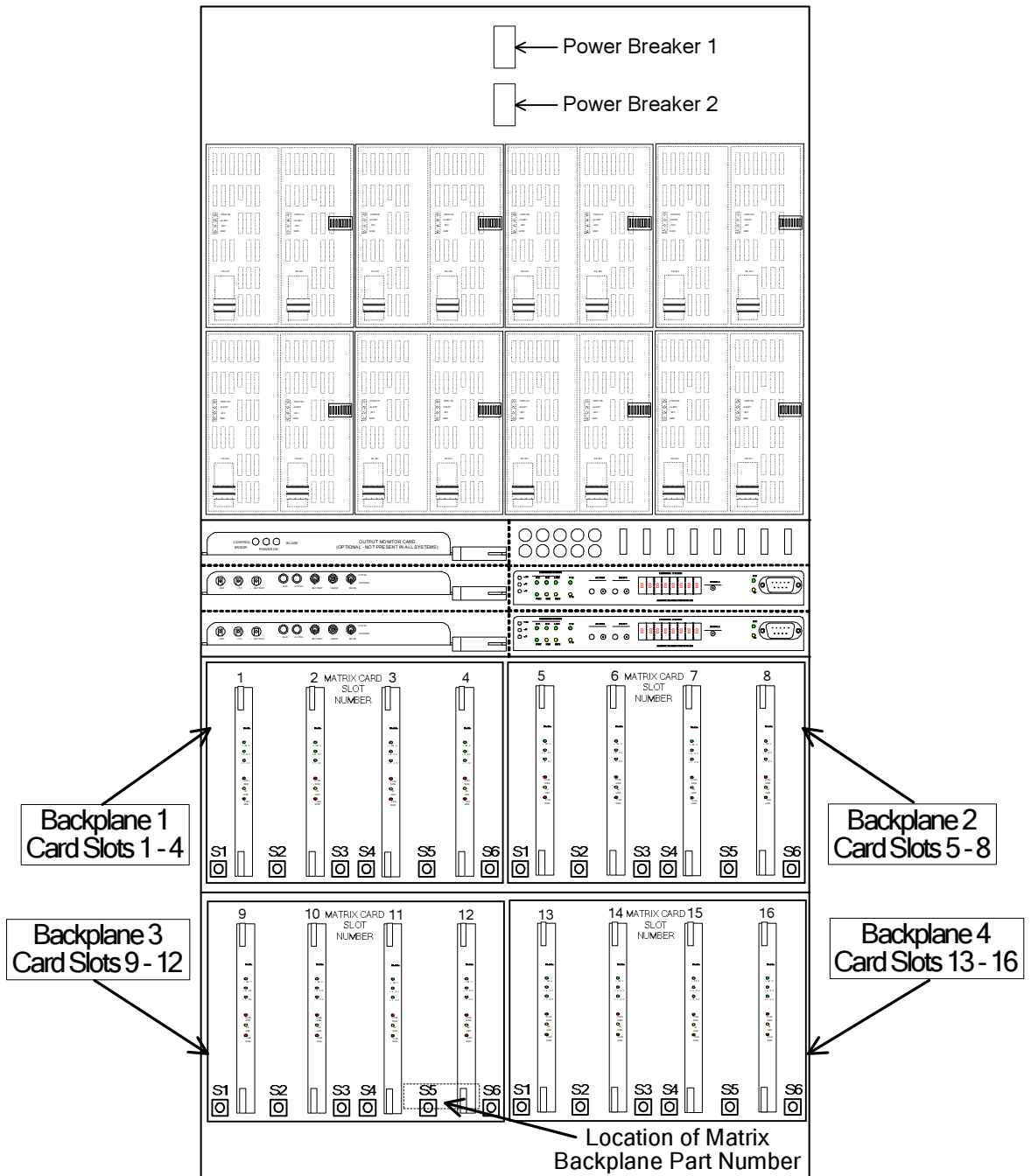
FIGURE 3-5: Matrix Backplane Rotary Switch Locations
