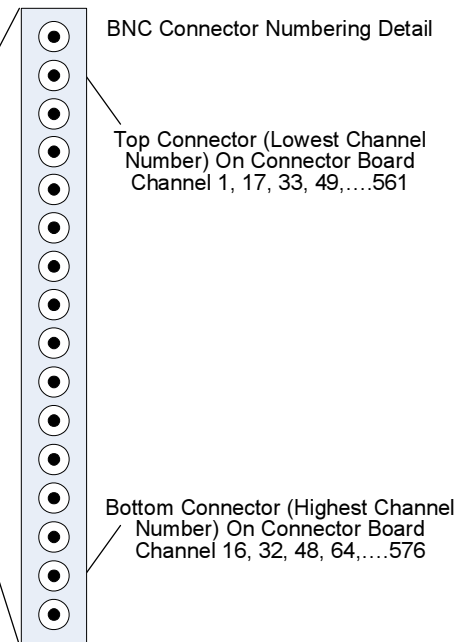
FIGURE 1-5: CHEETAH 576XR ROUTER CHASSIS (REAR VIEW)
