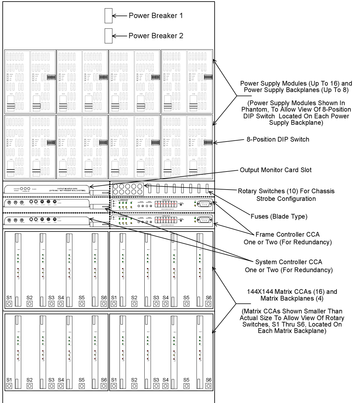
FIGURE 1-4 CHEETAH 576XR ROUTER CHASSIS (FRONT VIEW – DOOR OPEN)
