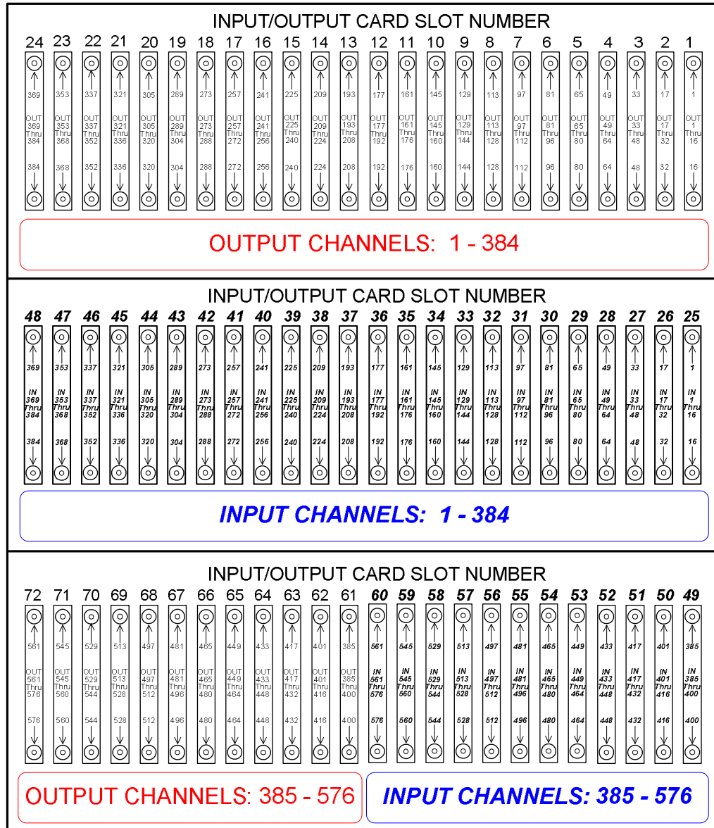
FIGURE 2-1: CHEETAH 576XR ROUTER INPUT/OUTPUT CONNECTOR ARRANGEMENT
