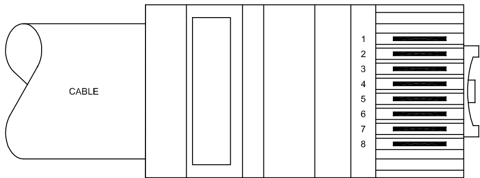
RJ-45 CONTACT SIDE SHOWN
