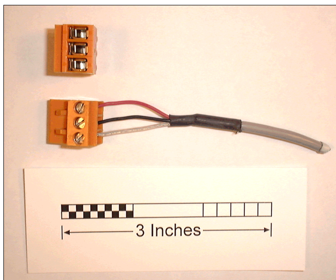
Figure 1. Audio Input Cable Connector Installation
