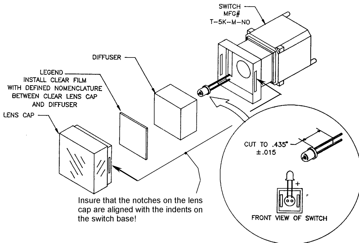
Legend Cap Breakaway Detail
