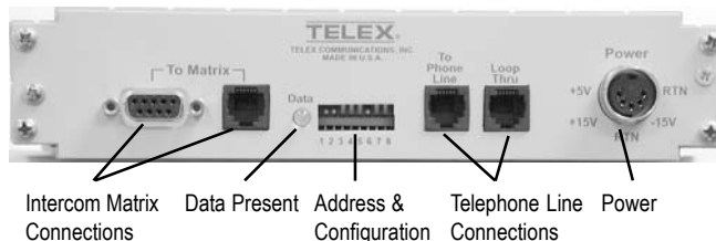
Figure 2 - TIF 2000 Rear Panel Features
