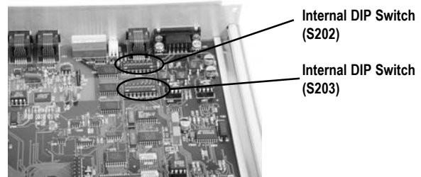
Figure 4 - TIF 2000 Internal DIP Switch Locations
