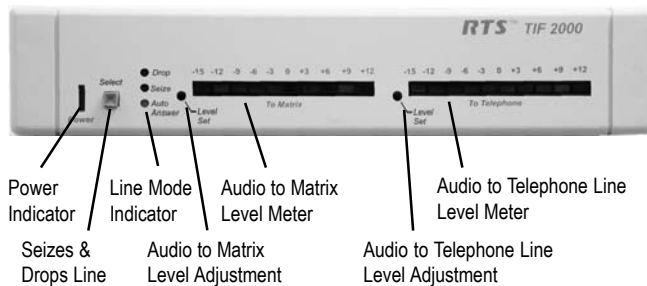
Figure 1 - TIF 2000 Front Panel Features
