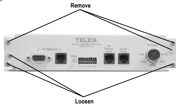
Figure 3 - TIF 2000 Internal DIP Switch Locations
