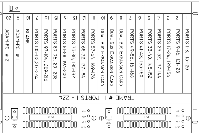
ADAM MATRIX FRAMES FRONT VIEW
