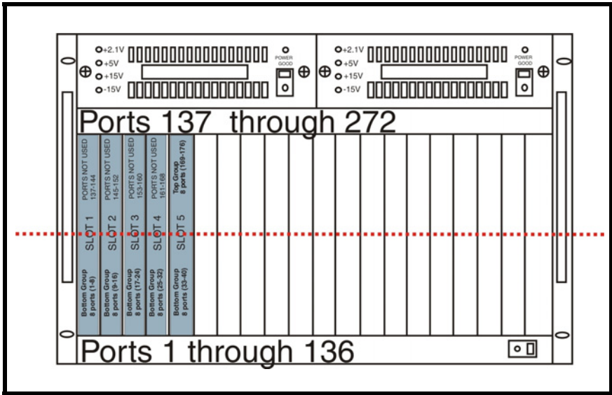
FIGURE 6. ADAM frame with both AIO-8 and AIO-16 cards.
