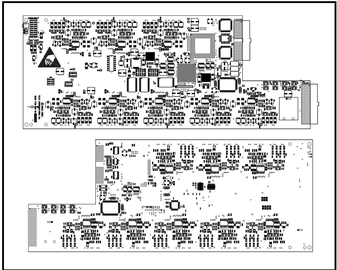
FIGURE 2. AIO-16 card top and bottom
