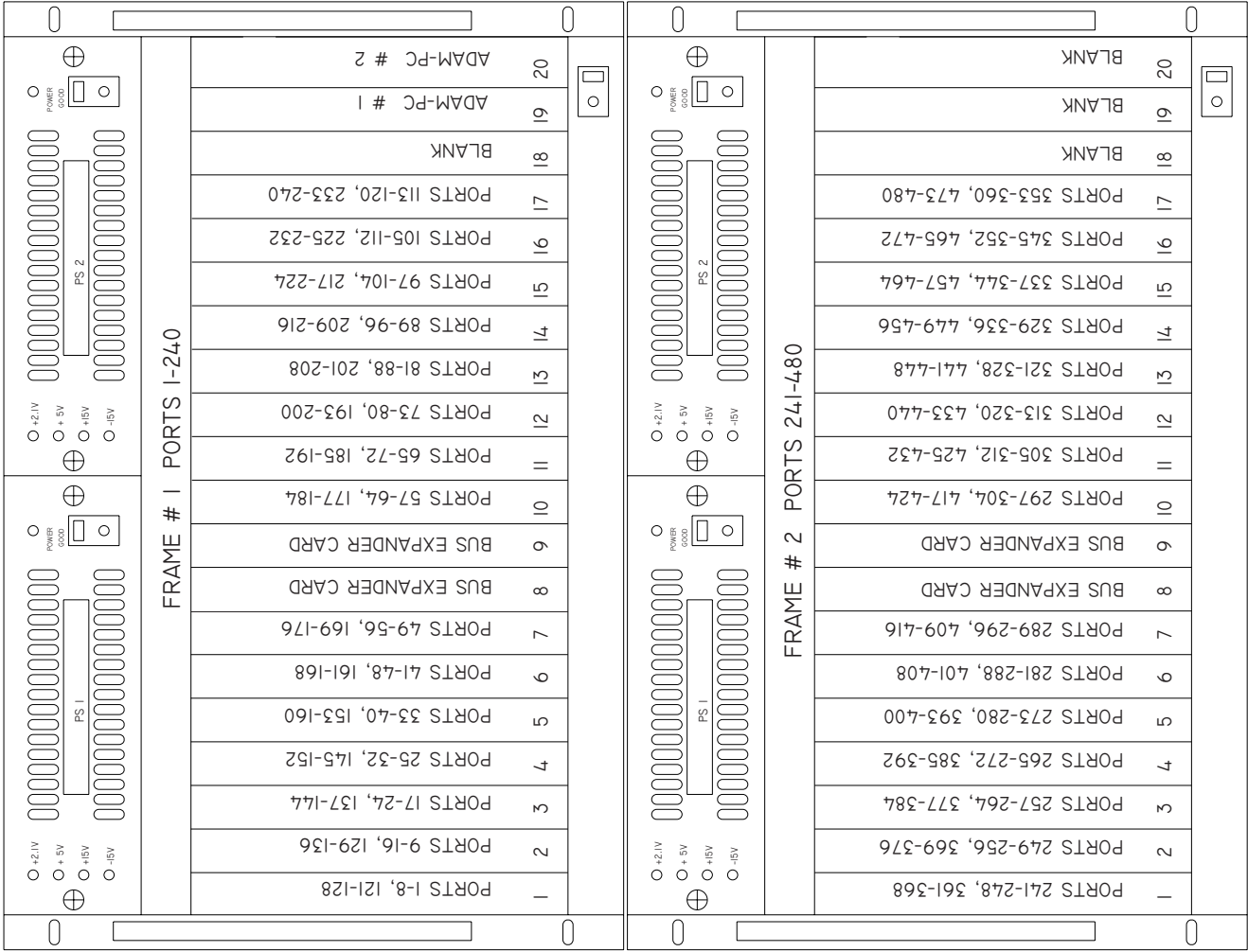
ADAM MATRIX FRAMES FRONT VIEW
