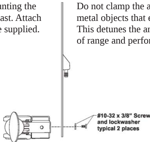
Figure 5 Clamps
