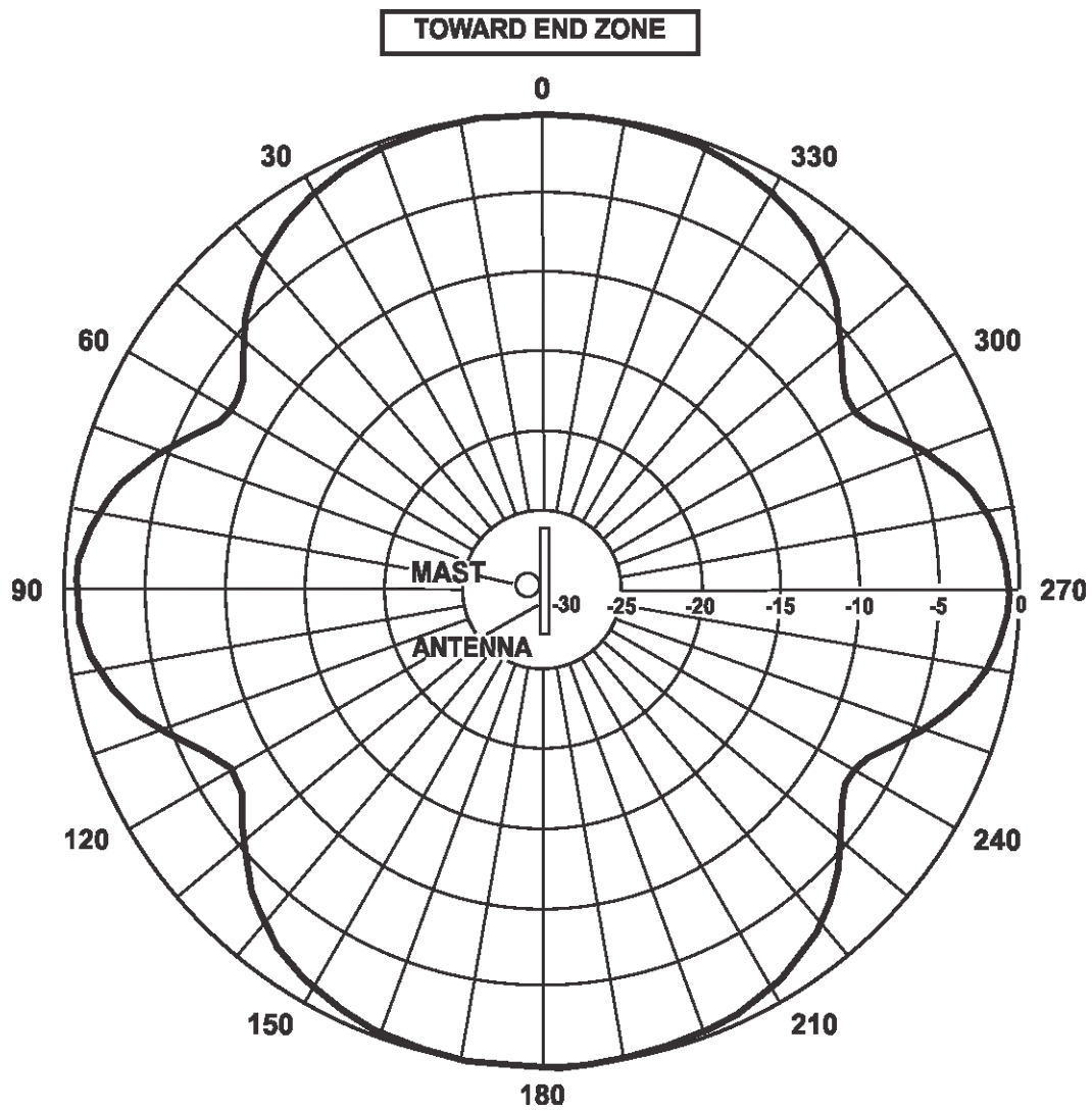
Figure 4 Typical ALP-700 UHF Bi-directional Antenna Pattern
