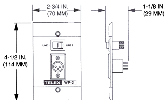
Dimensions (WP-2 Shown)
