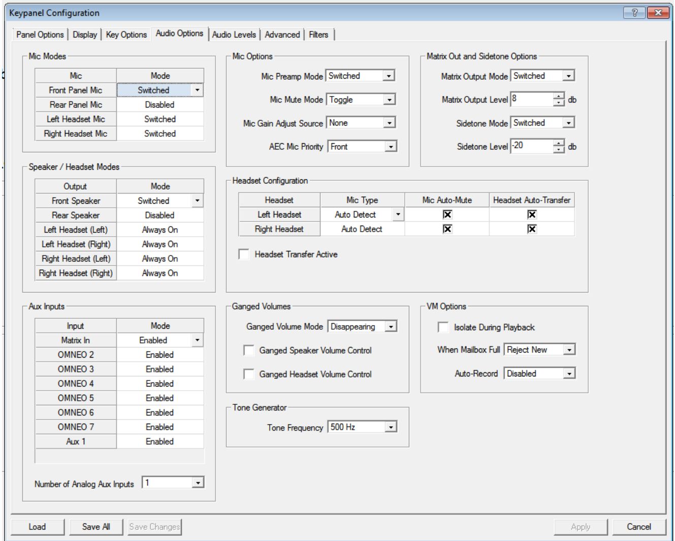
FIGURE 54. Keypanel Configuration – Audio Options
