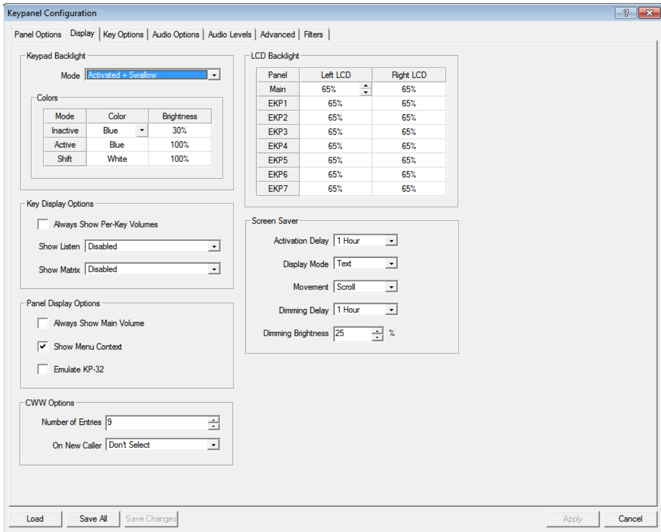
FIGURE 36. Keypanel Configuration – Display Page
