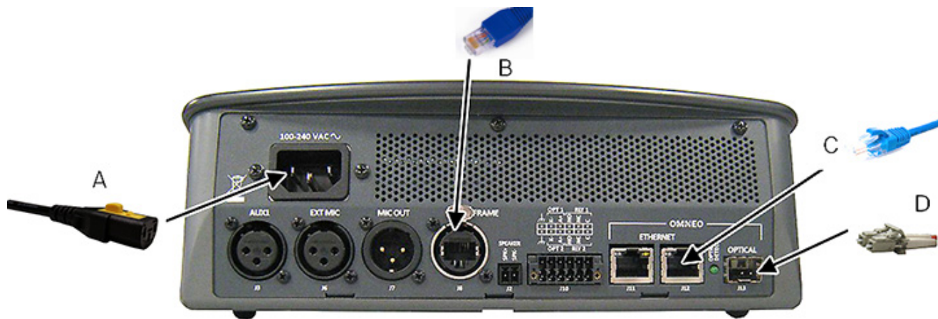
FIGURE 3. DKP-4016 Installation
