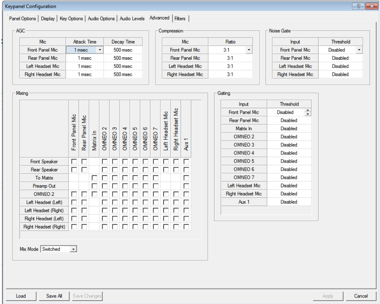
FIGURE 72. Keypanel Configuration – Advanced
