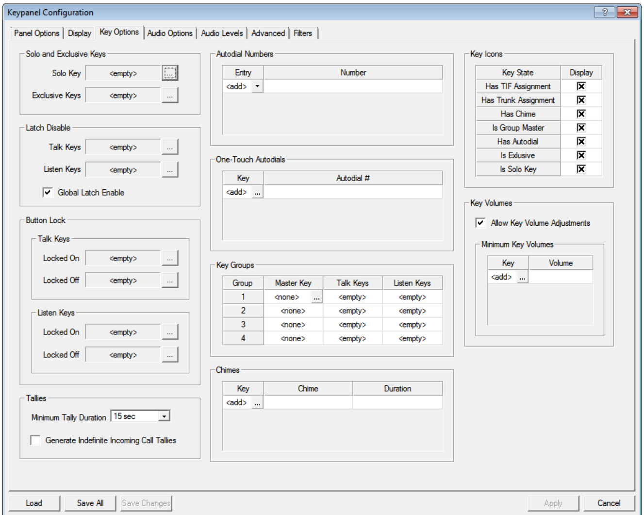
FIGURE 43. Keypanel Configuration – Key Options Page
