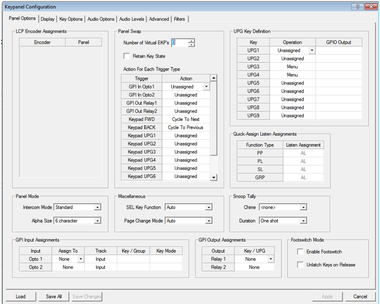
FIGURE 26. Keypanel Configuration – Panel Options
