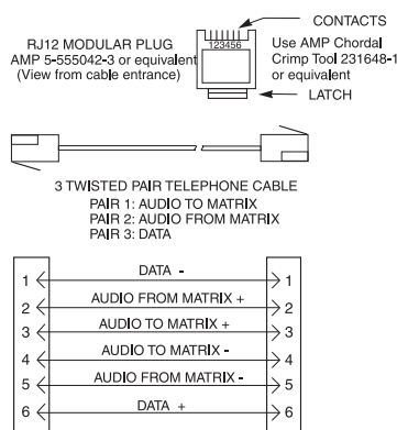
FIGURE 20. RJ12 Intercom Cable Wiring
