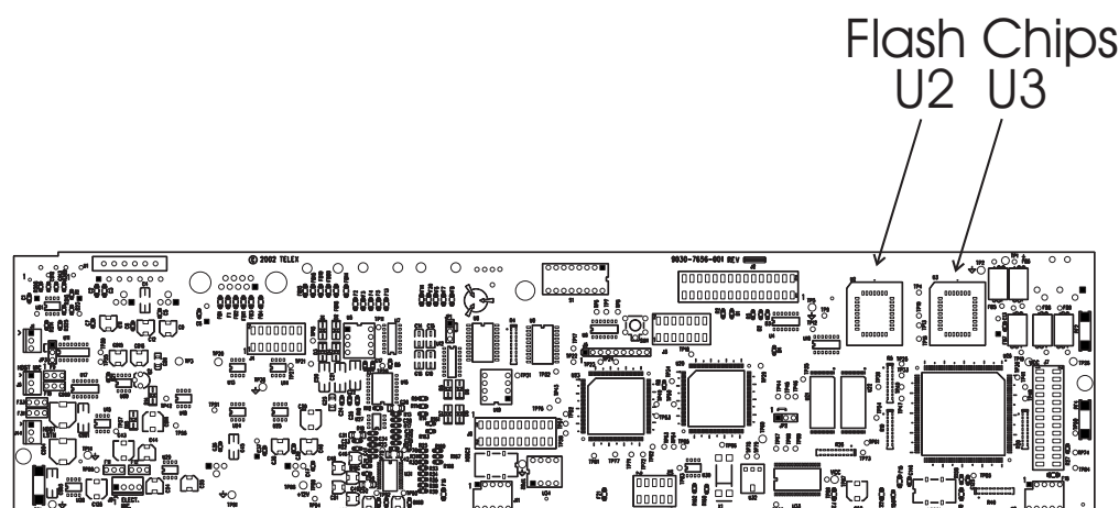
FIGURE 23. Flash Chip placement on the KP-32 motherboard
