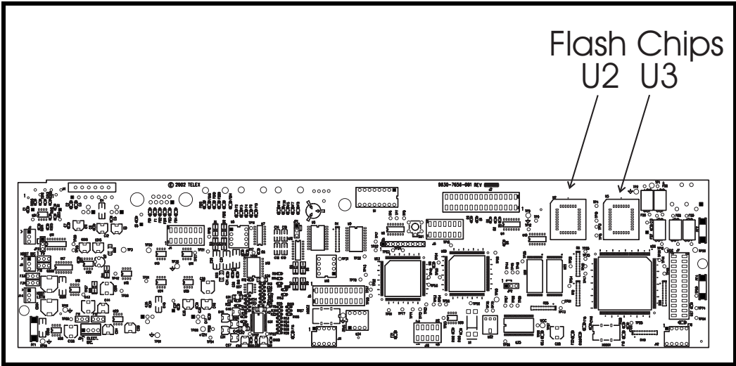
Figure 1. Flash Chip placement on the KP-32 motherboard
