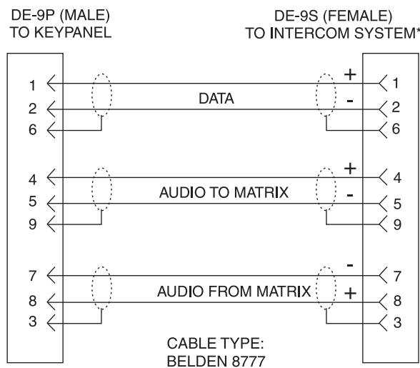
Figure 2.2 DE9S Intercom Cable Wiring
