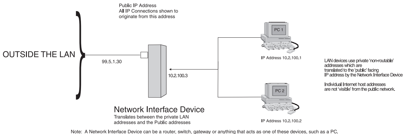
Figure 3. Network Address Translation
