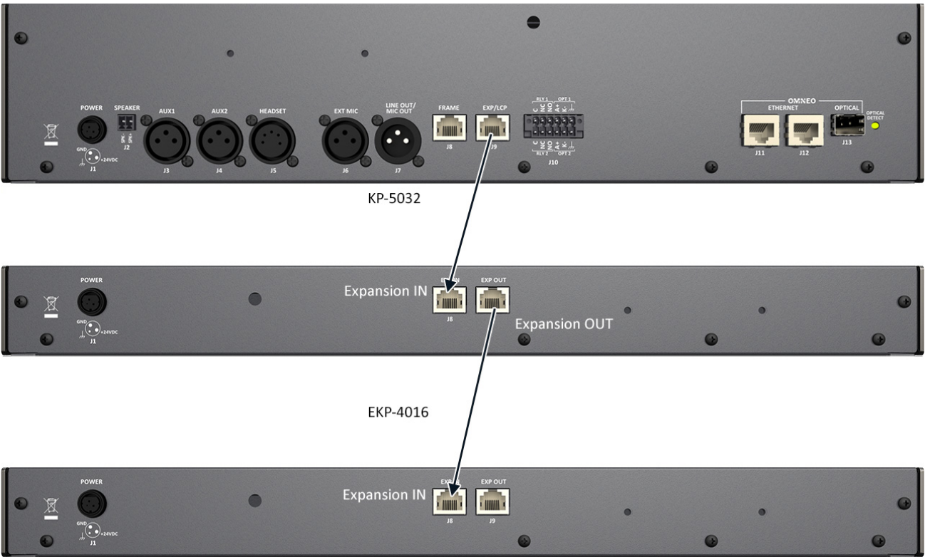
FIGURE 91. Expansion Panel Cabling
