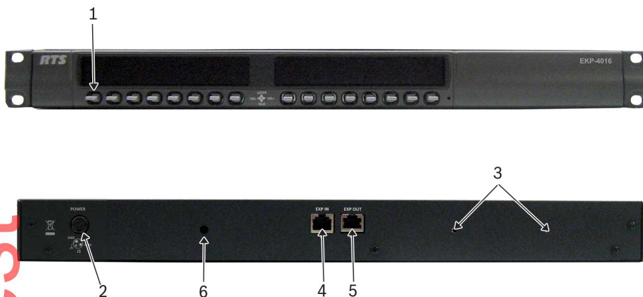
FIGURE 90. EKP-4016 Expansion Panel Reference View - Front and Rear
