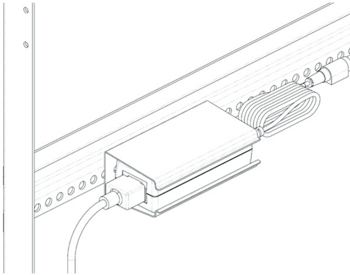
FIGURE 92. Mounting Bracket – Horizontal on a Crossbar
