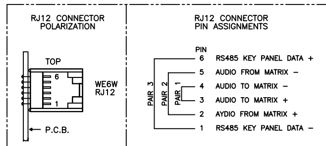
AIO-BC-8-RJ12 Back Card Part # 90007688000
