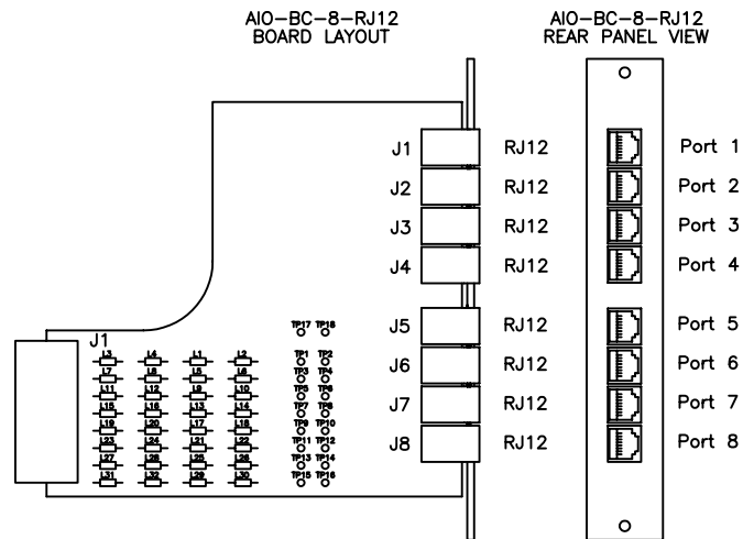
AIO-BC-8-RJ12 Back Card Part # 90007688000
