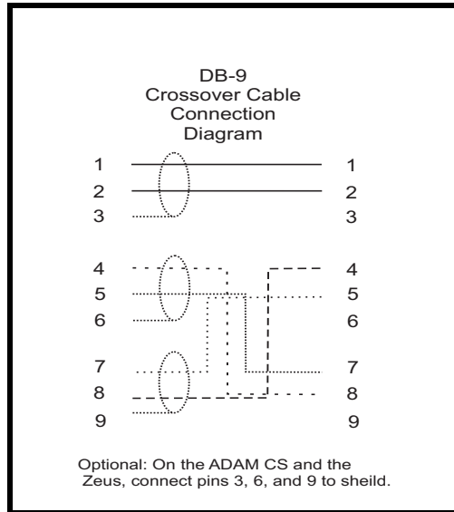
FIGURE 2. DB-9 Crossover Cable Connection Diagram
