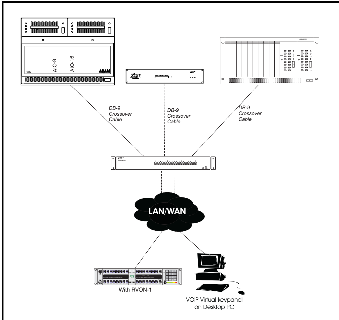
FIGURE 6. Remote Mode - Remote Mode means the keypanels are not connected to the RVON-I/O directly. In the example, the KP-32 with RVON-1 or the VKP has to pass through the LAN/WAN before connecting to the RVON-I/O.
