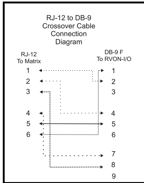
FIGURE 3. RJ-12 to DB-9 Crossover Cable Connection Diagram
