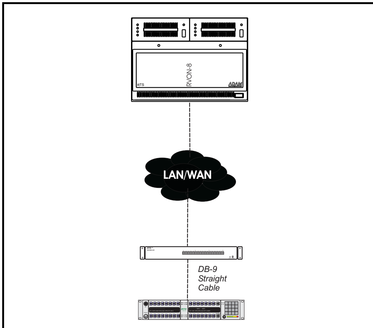
FIGURE 5. Local Mode - This system diagram shows Local mode. It is called local mode because the keypanel is connected directly to the RVON-I/O.
