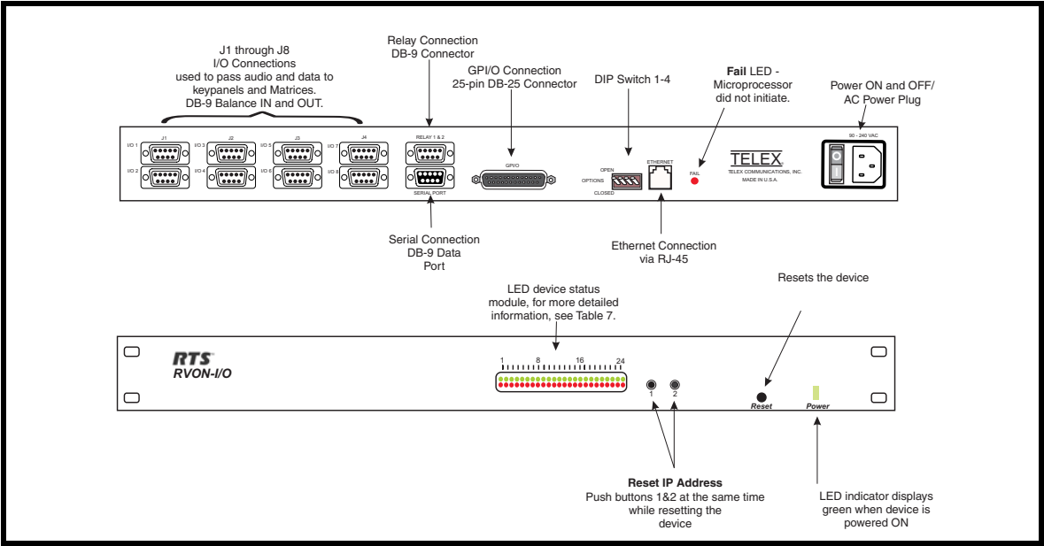
FIGURE 1. RVON-I/O Reference View
