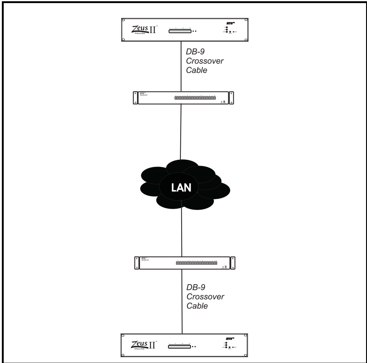
FIGURE 8. Trunking with RVON-I/O - When you trunk two intercom systems together using two RVON-I/O's, you can configure one as Remote and the other as Local. However, remote to remote setup is the preferred system setup for trunking.
