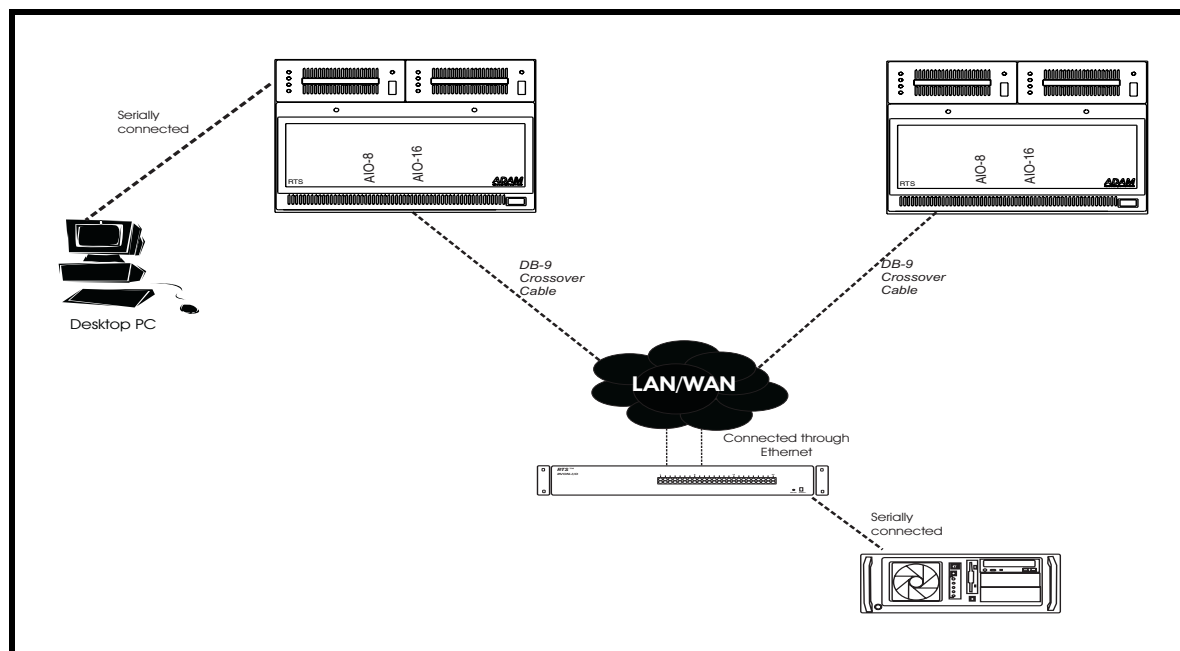
FIGURE 4. Serial Pass-Through system diagram
