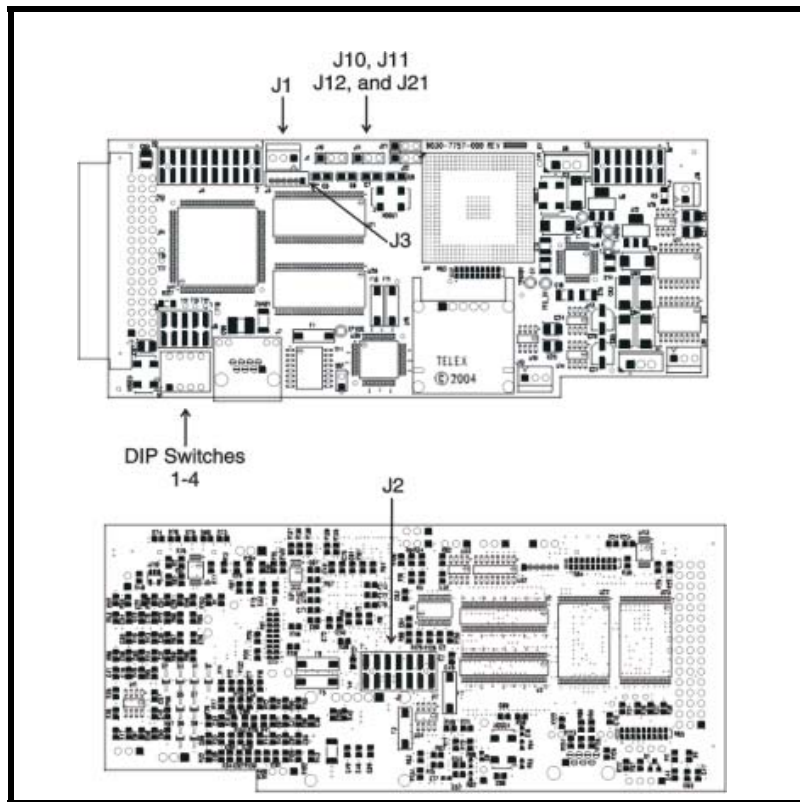
FIGURE 9. Front and back of the RVON-1 board
