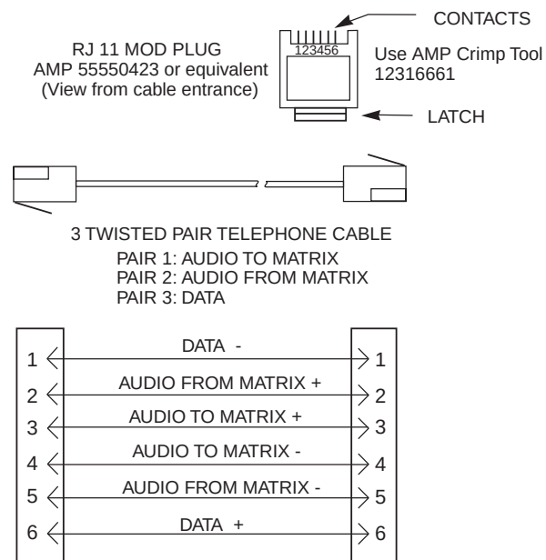
Figure 2. RJ-11 Intercom cable wiring diagram
