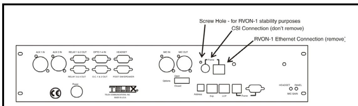
Figure 2. Knock out positions for the RVON-1 card on the KP-32
