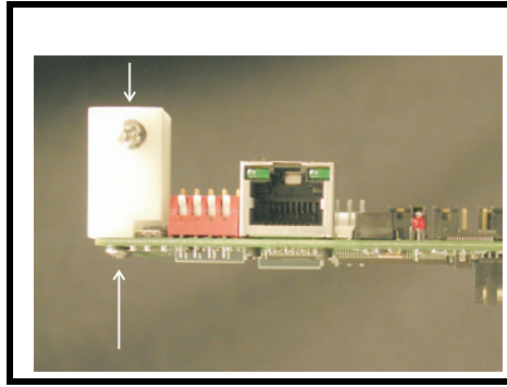
Figure 3. The placement of the spacer and screw position on the RVON-1 card.
