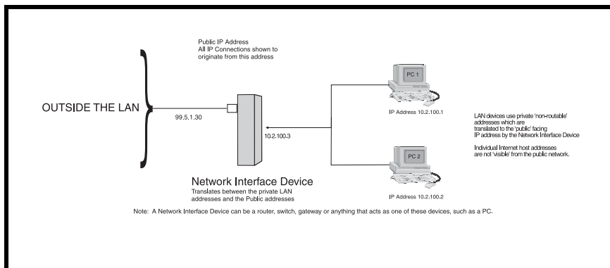
Figure 6. Network Address Translation
