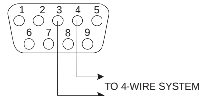
TO SSA-424 AUX CONNECTOR DB9F CABLE CONNECTOR PIN NUMBERS (View from solder or crimp side)
