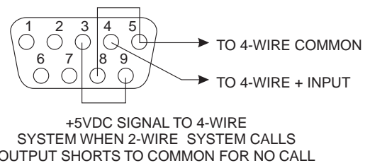
Figure 7. Call signal connections for a 4-wire intercom system other than ADAM, ADAM CS, and Zeus.
