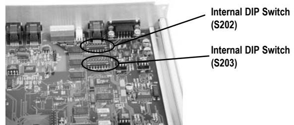
Figure 4 - TIF 2000 Internal DIP Switch Locations
