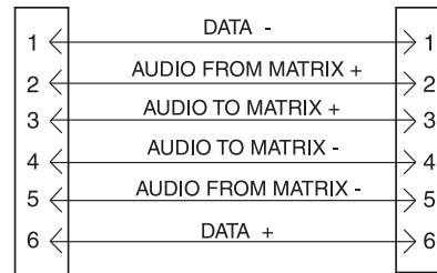
Figure 6 - RJ12 Intercom Cable
