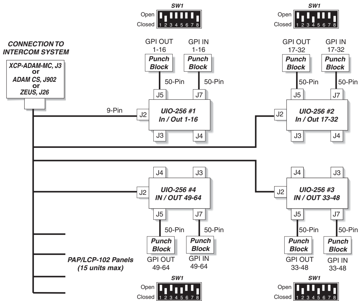
Figure 2. Multi-Drop Connections
