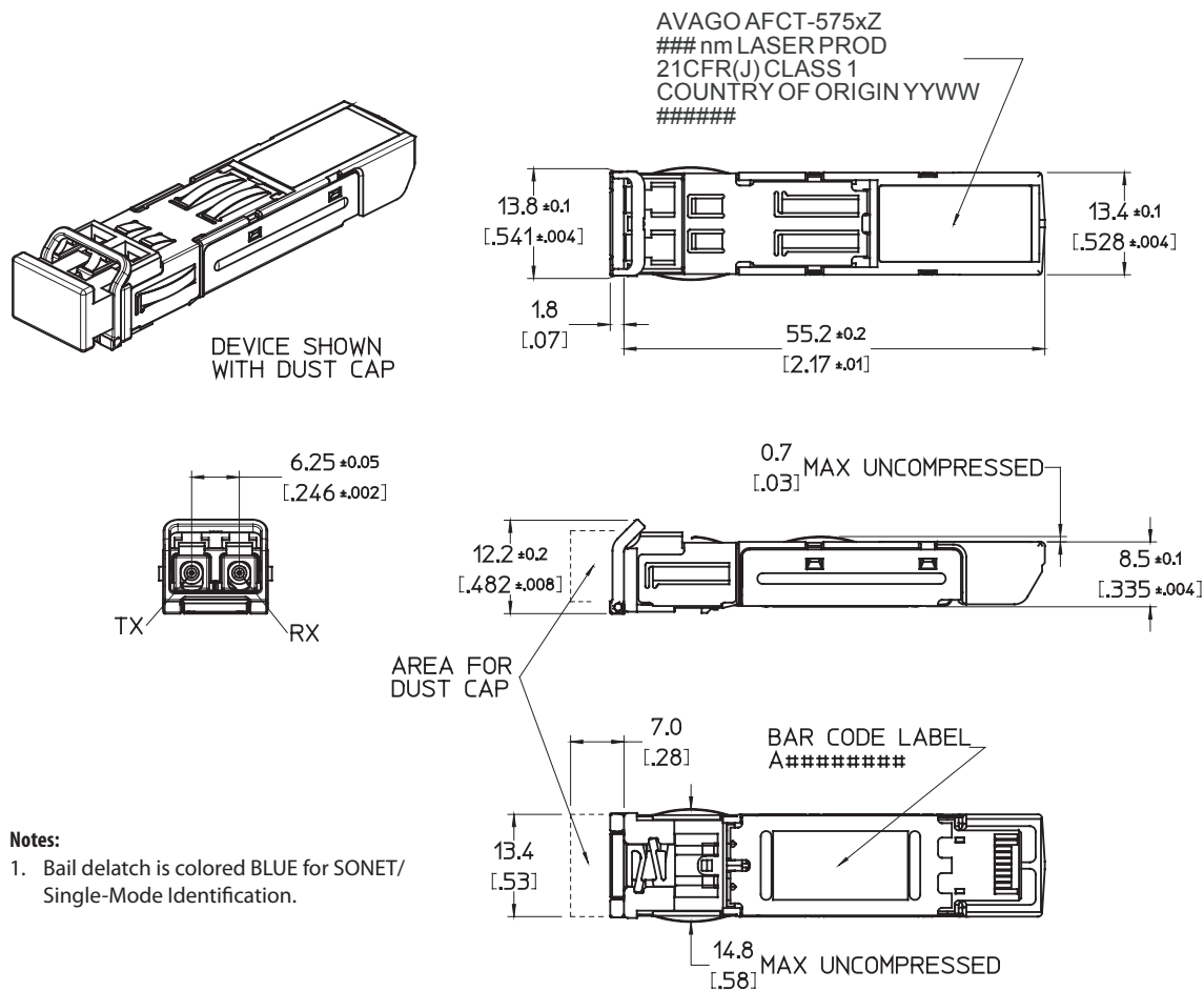
Figure 6. Module Drawing
