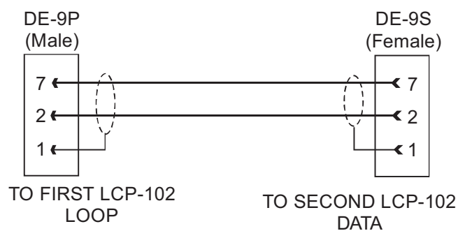
Figure 5. Cable to interconnect two LCP-102's (All intercom systems)
