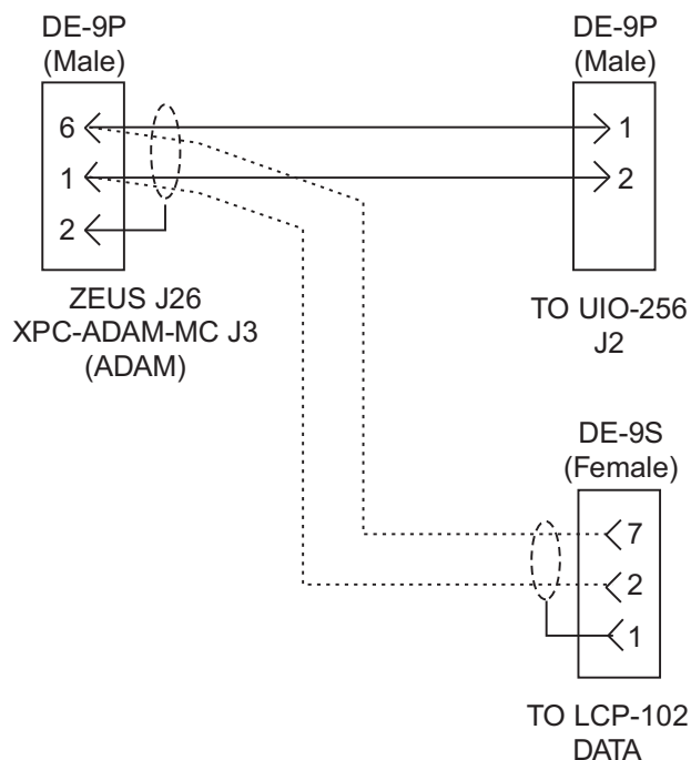
Figure 4. "Y" cable for connection of an LCP-102 and a UIO-256 to a Zeus or ADAM Intercom System
