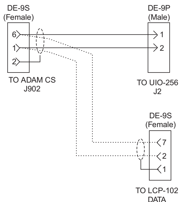
Figure 7. "Y" cable for connection of an LCP-102 and a UIO-256 to an ADAM CS Intercom System
