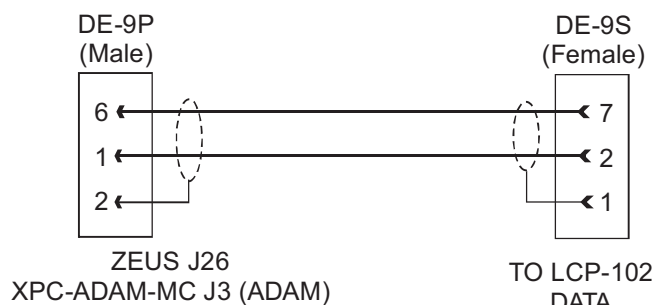
Figure 3. Interconnect cable from a Zeus or ADAM Intercom System to the LCP-102
