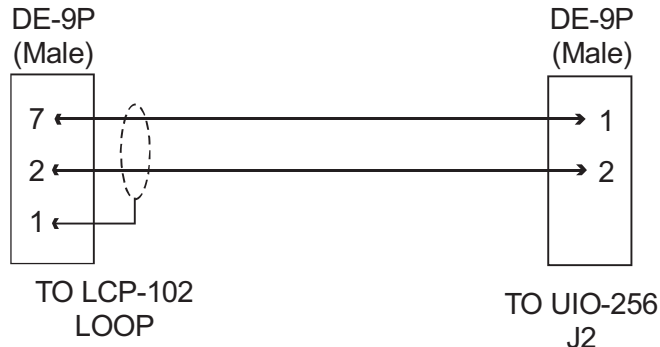
Figure 8. Cable to connect a UIO-256 to the LCP-102 (All intercom systems)
