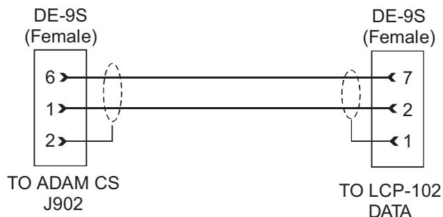
Figure 6. Interconnect cable from an ADAM CS Intercom System to the LCP-102
