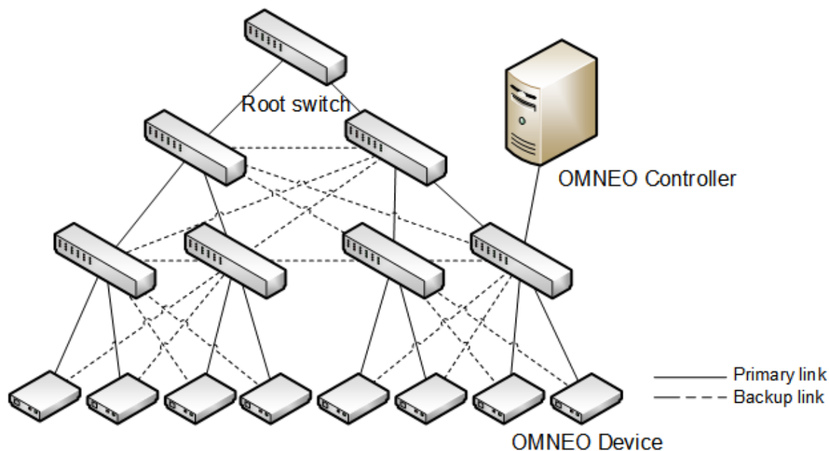
FIGURE 13. Tree Redundant
