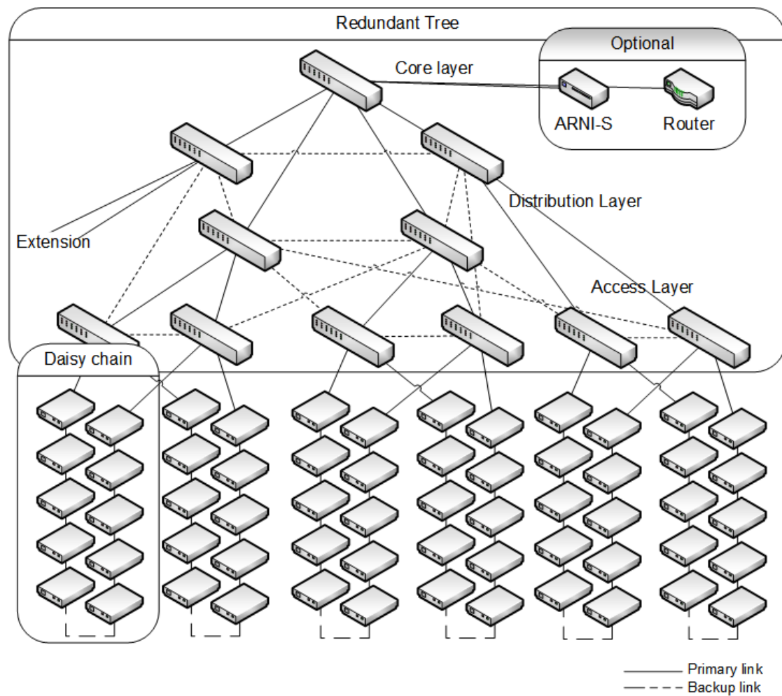
FIGURE 14. Mesh Half-Redundant
