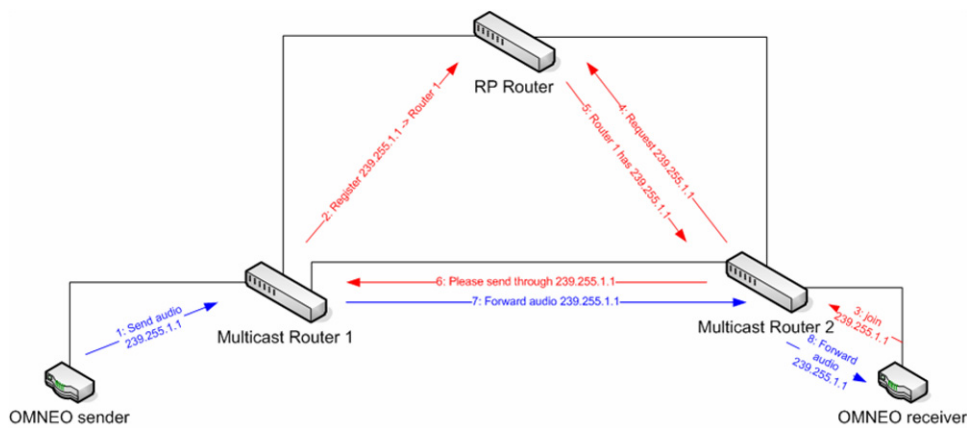
FIGURE 16. PIM-SM Example
