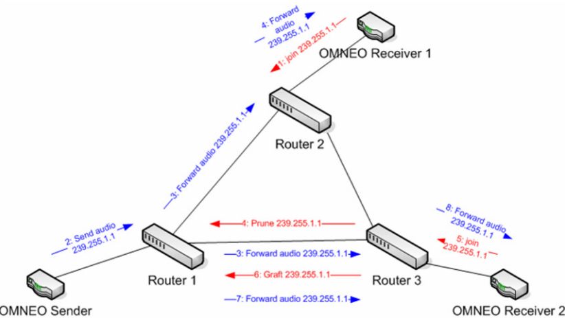
FIGURE 17. PIM-DM Example
