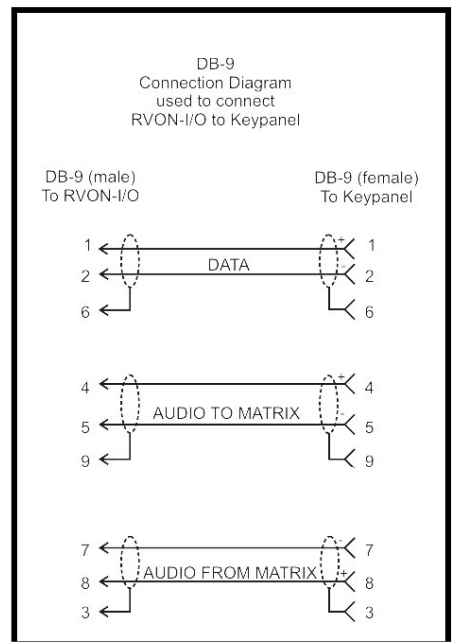
FIGURE 7. Straight DB-9 to DB-9 Connection Diagram
