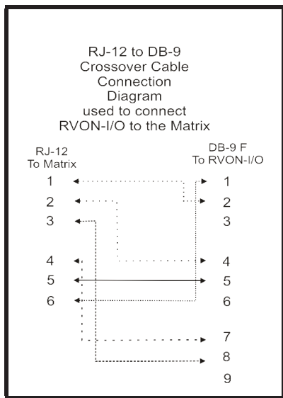
FIGURE 3. RJ-12 to DB-9 Crossover Cable Connection Diagram
