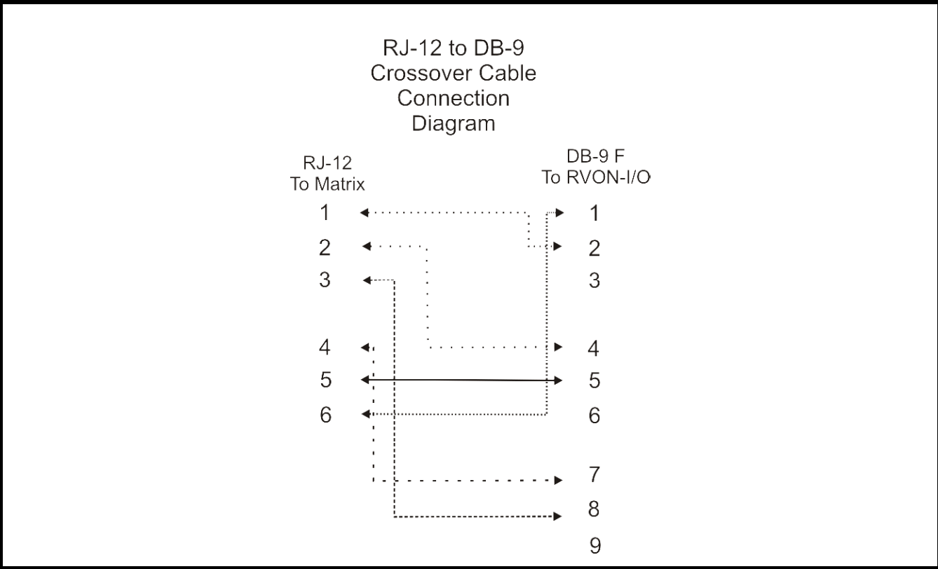
FIGURE 3. RJ-12 to DB-9 Crossover Cable Connection Diagram
