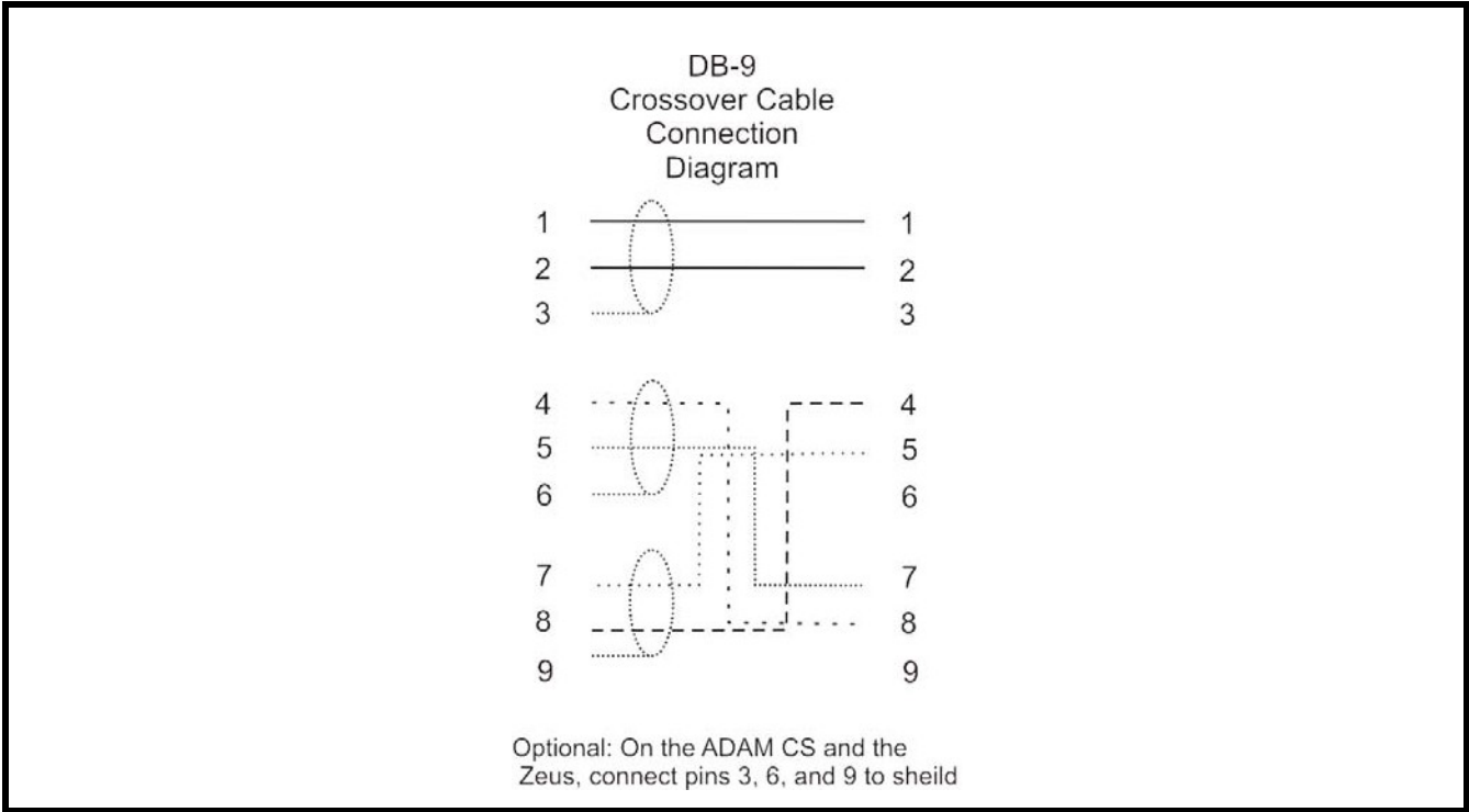
FIGURE 2. DB-9 Crossover Cable Connection Diagram
