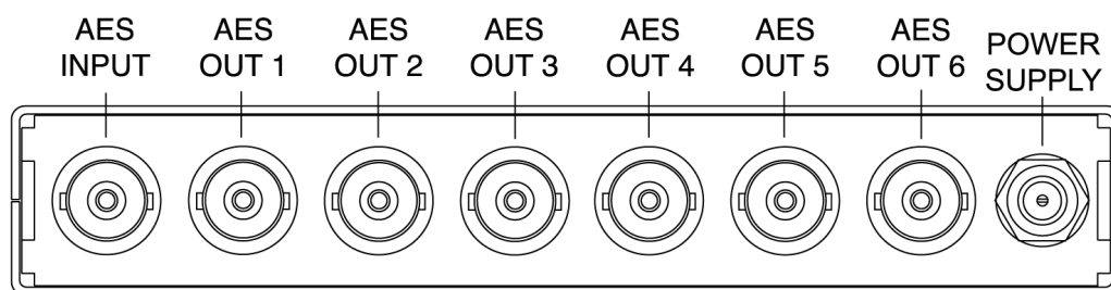
Figure 8. ADA-9503 Rear Connections Configuration
