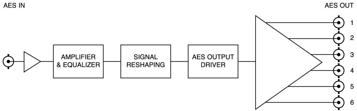
Figure 1. Simplified Block Diagram of ADA-9503 Functions
