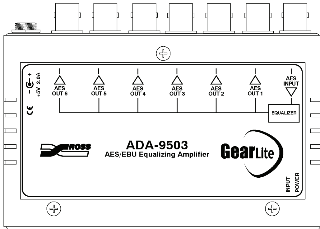
Figure 7. ADA-9503 Cable Connections Indicator Label
