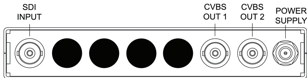
Figure 8. CMA-9011 Rear Connections Configuration
