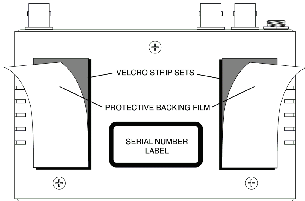
Figure 2. Velcro Installation Option
