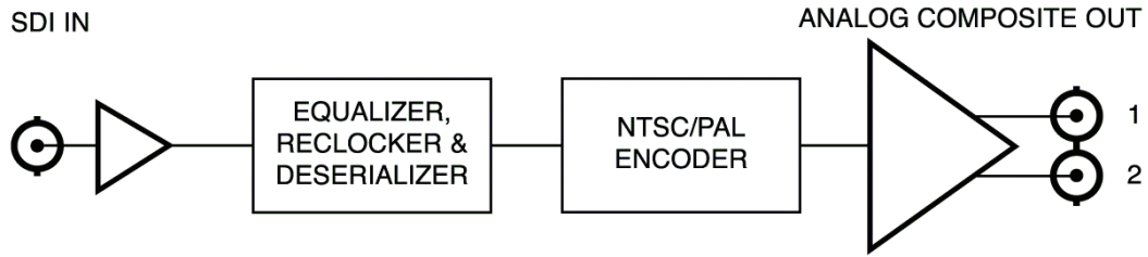
Figure 1. Simplified Block Diagram of CMA-9011 Functions
