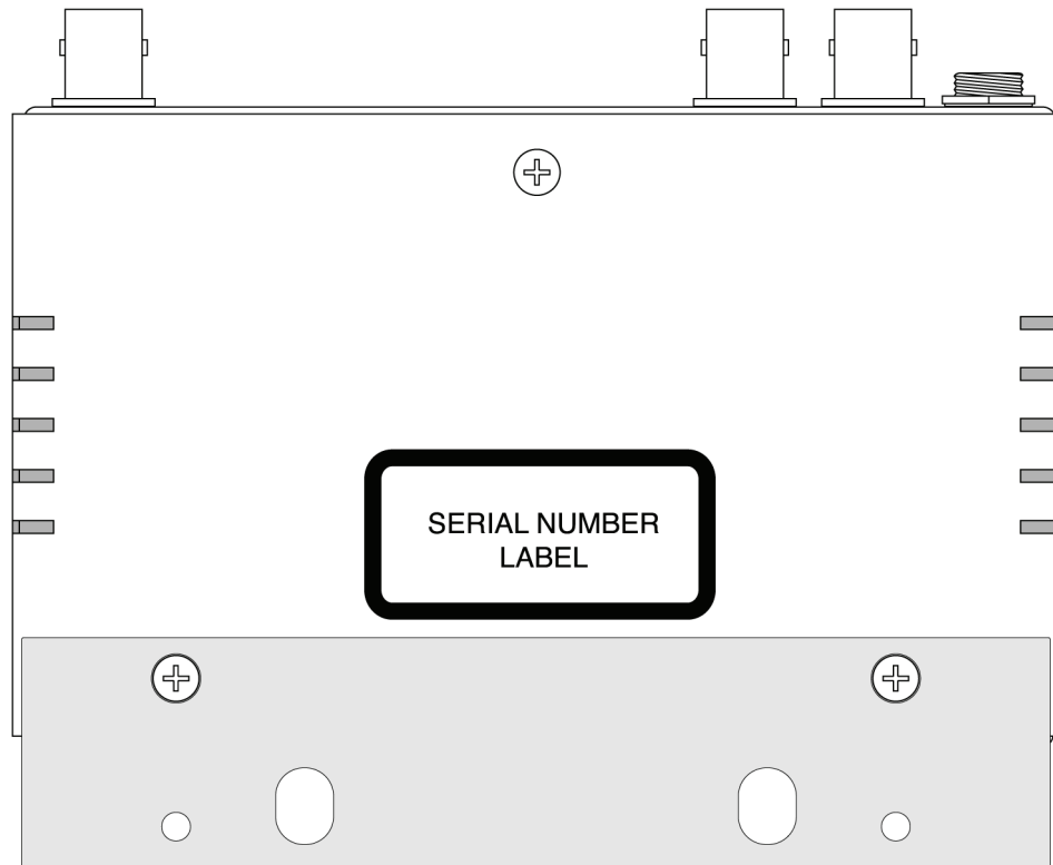
Figure 3. Flat Metal Plate Installation Option
