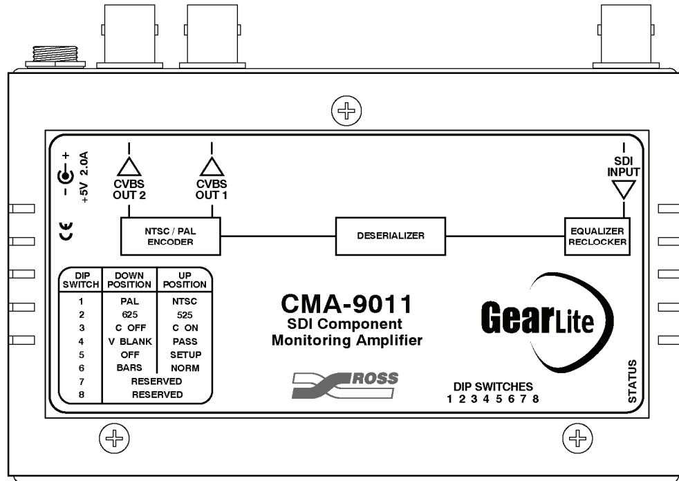
Figure 7. CMA-9011 Cable Connections Indicator Label
