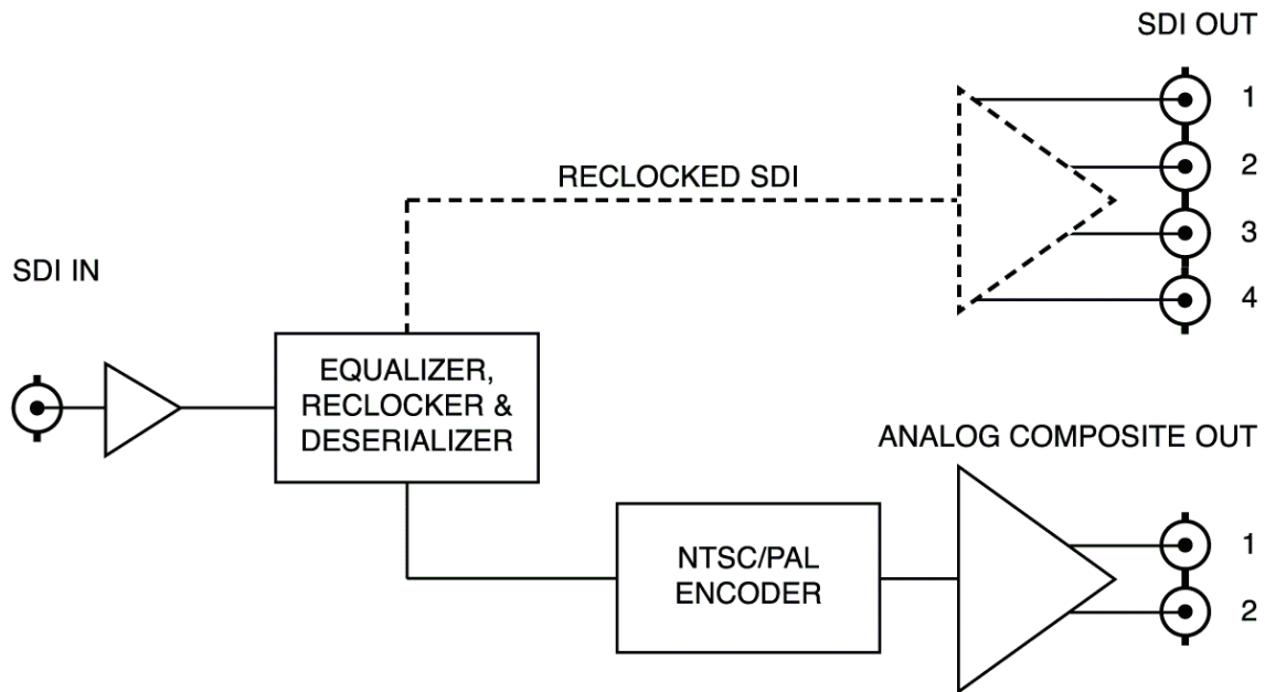
Figure 1. Simplified Block Diagram of CMA-9011-R Functions
