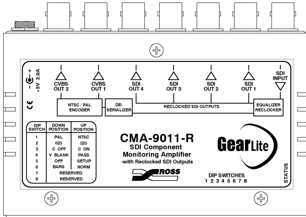
Figure 7. CMA-9011-R Cable Connections Indicator Label
