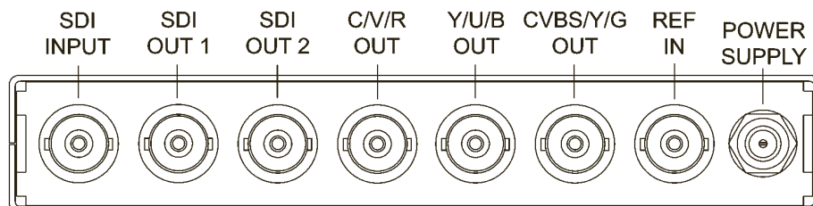
Figure 8. DAC-9013-R Rear Connections Configuration
