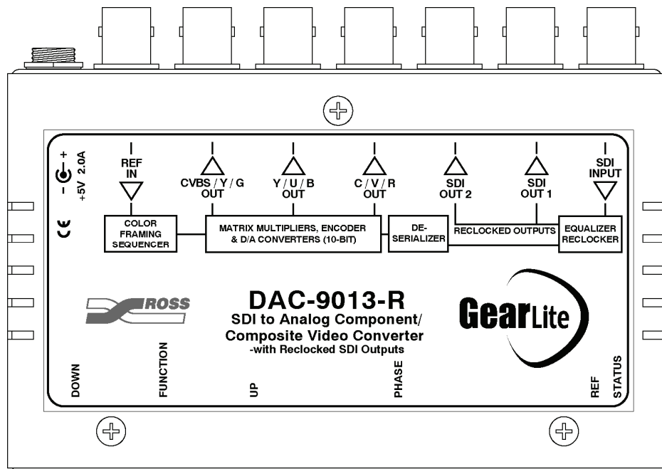
Figure 7. DAC-9013-R Cable Connections Indicator Label
