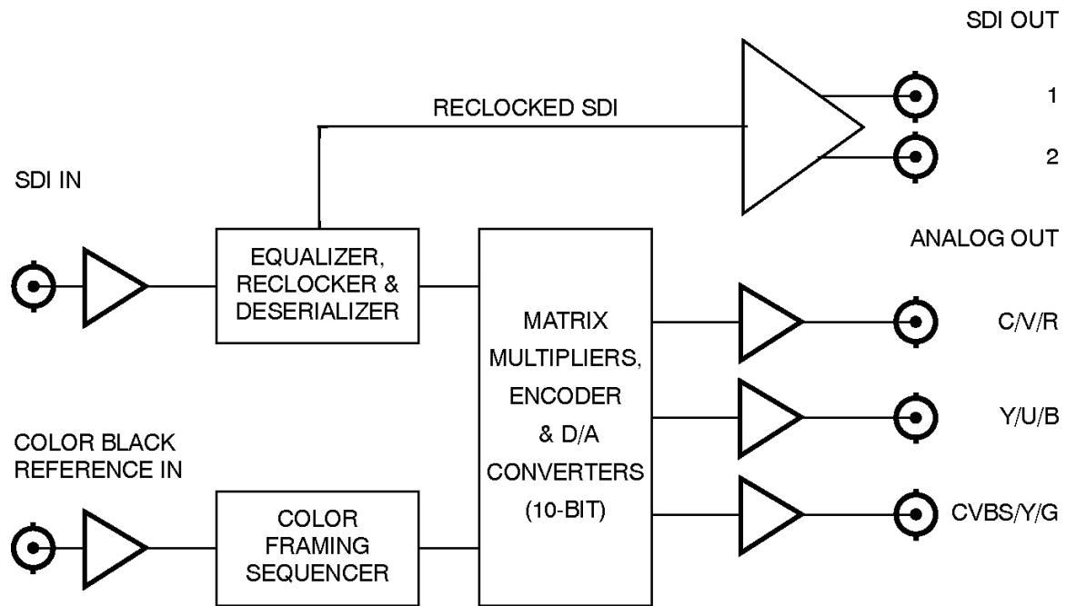
Figure 1. Simplified Block Diagram of DAC-9013-R Functions
