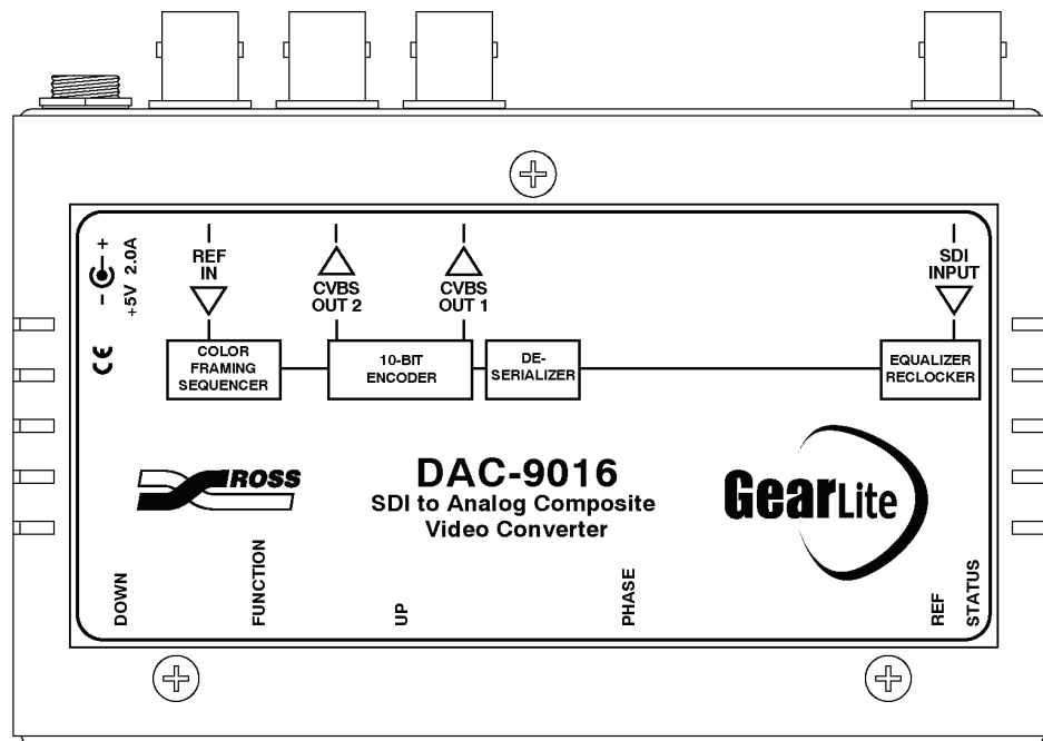
Figure 7. DAC-9016 Cable Connections Indicator Label
