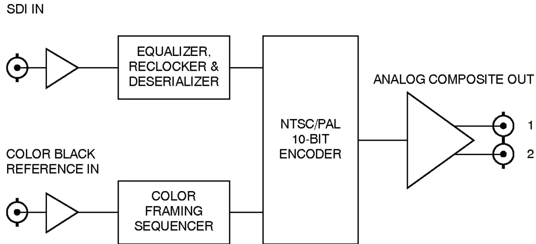
Figure 1. Simplified Block Diagram of DAC-9016 Functions
