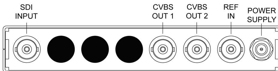
Figure 8. DAC-9016 Rear Connections Configuration
