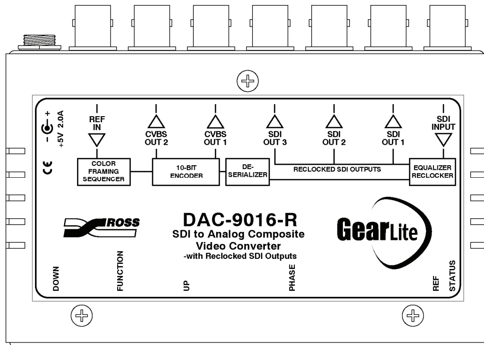
Figure 7. DAC-9016-R Cable Connections Indicator Label
