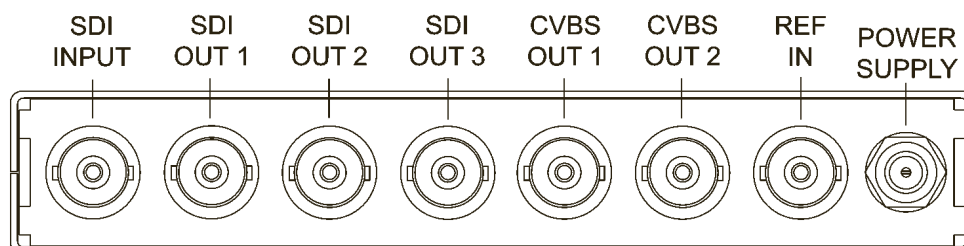
Figure 8. DAC-9016-R Rear Connections Configuration
