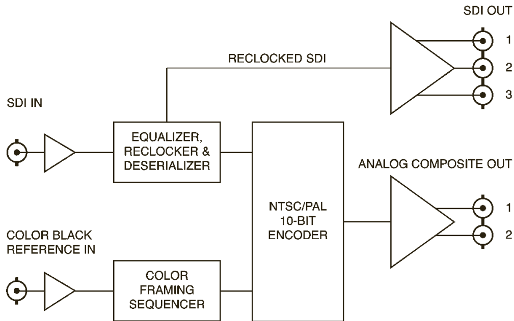
Figure 1. Simplified Block Diagram of DAC-9016-R Functions
