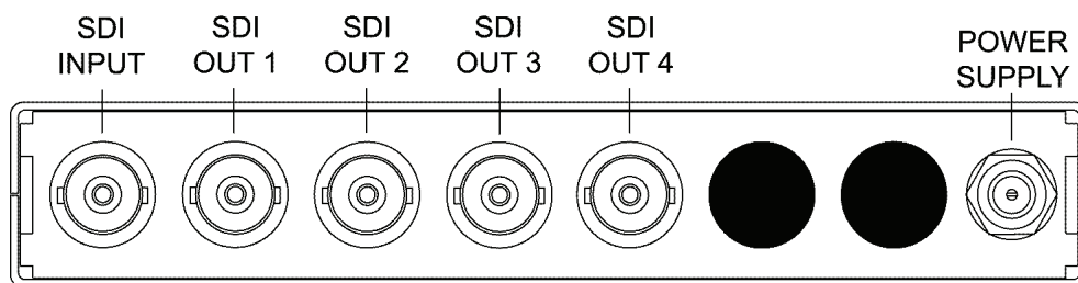
Figure 8. SEA-9003 Rear Connections Configuration
