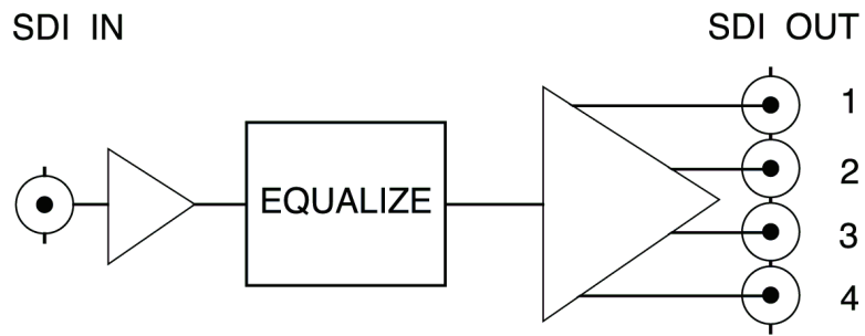
Figure 1. Simplified Block Diagram of SEA-9003 Functions
